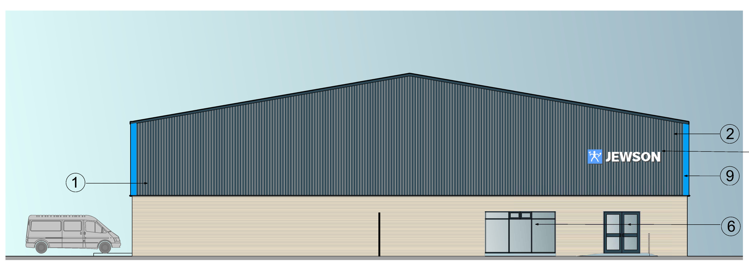
NORTH ELEVATION
