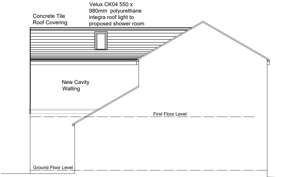
South Elevation (Side)
