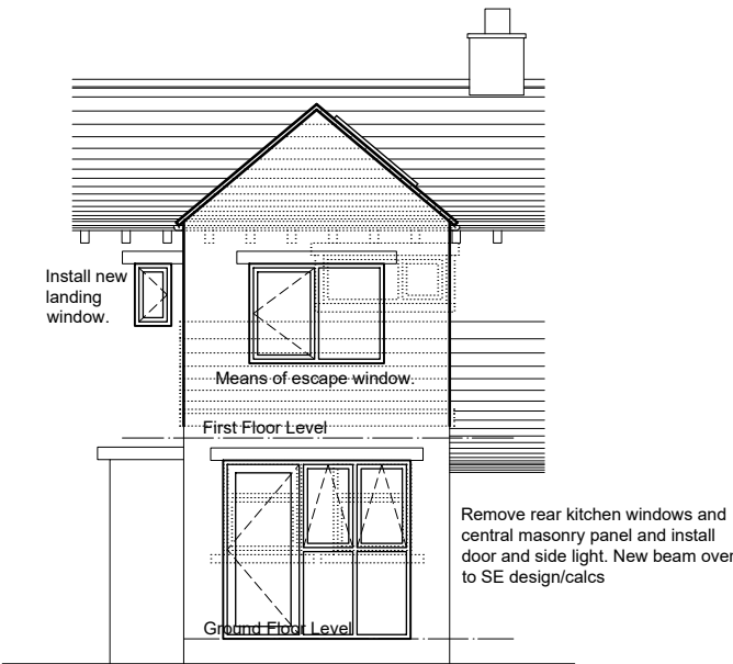
West Elevation (rear)
