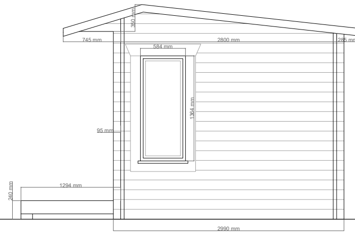
SIDE ELEVATION RIGHT
