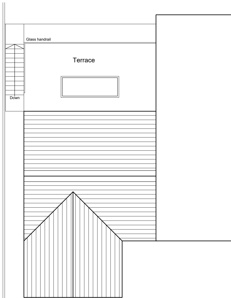
Roof Plan
