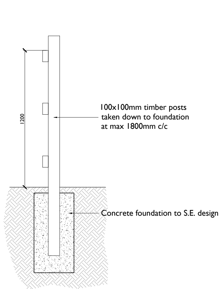
Section
