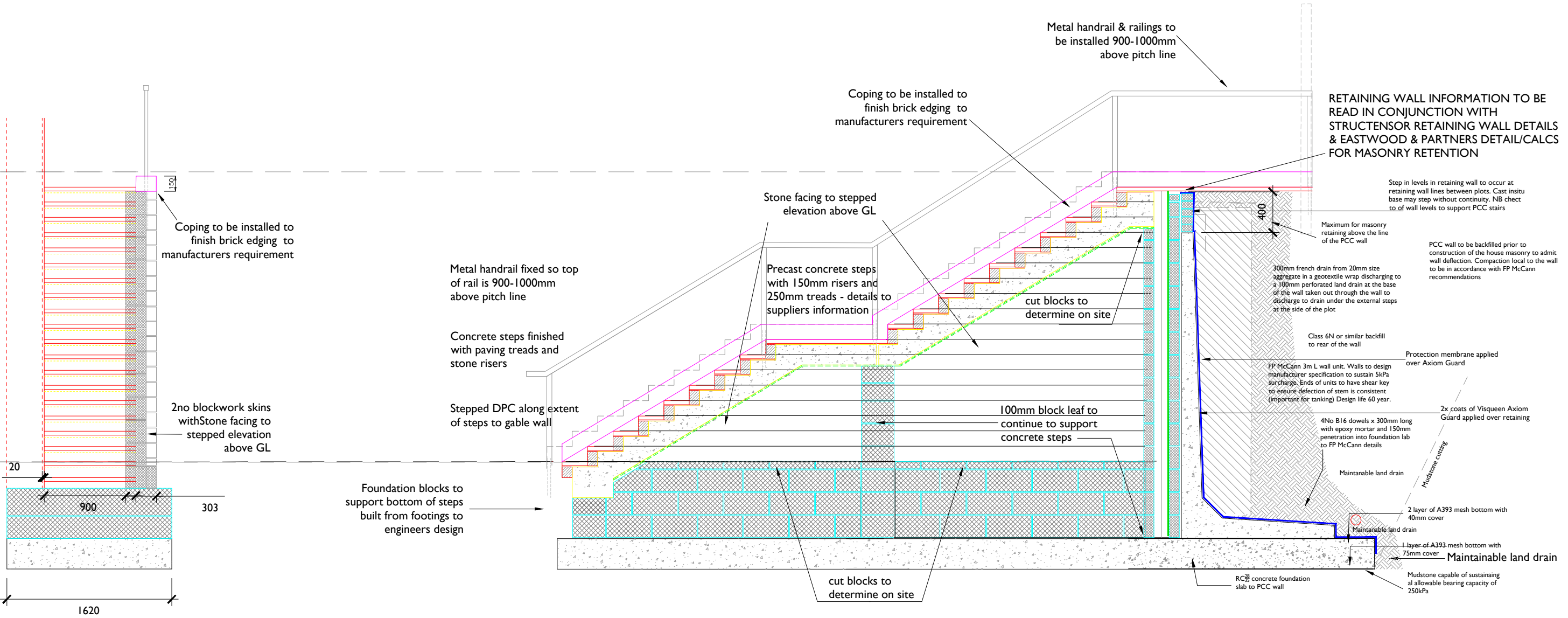
FRONT ELEVATION: SINGLE STAIR DESIGN
