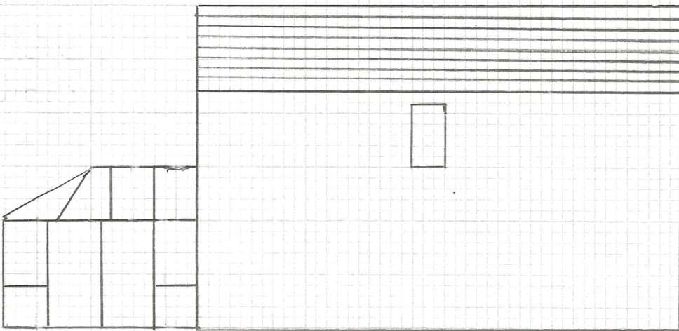
West 1:100
