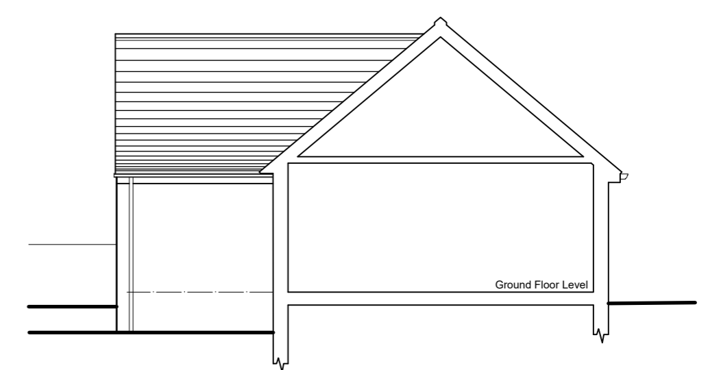
South East Sectional Elevation (side)
