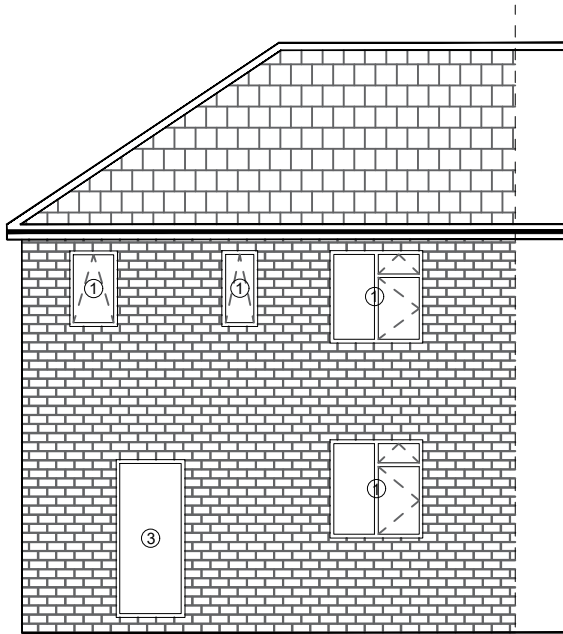
EXISTING REAR ELEVATION (North East)
