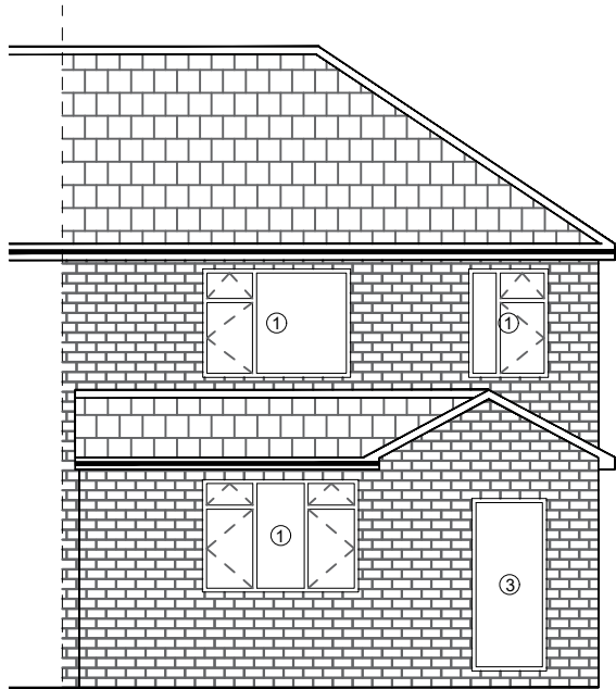
EXISTING FRONT ELEVATION (South West)
