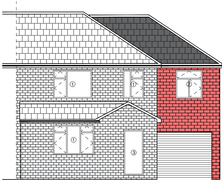
PROPOSED FRONT ELEVATION (South West)
