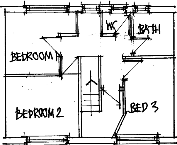
PROPOSED FIRST FLOOR
