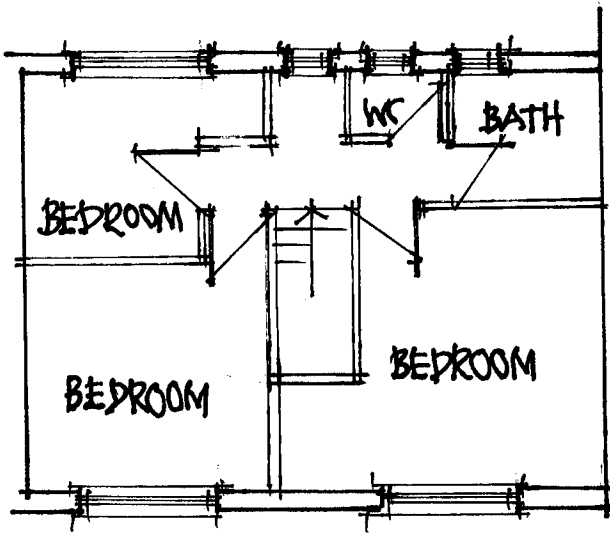
EXISTING FIRST FLOOR
