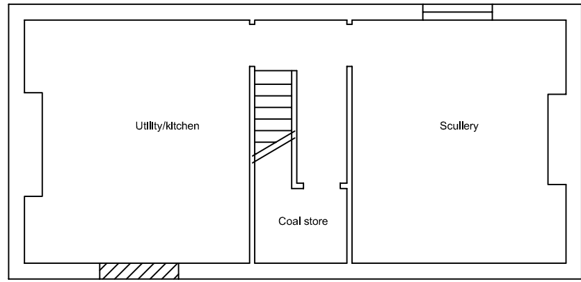
Existing Basement 1:100@A1
