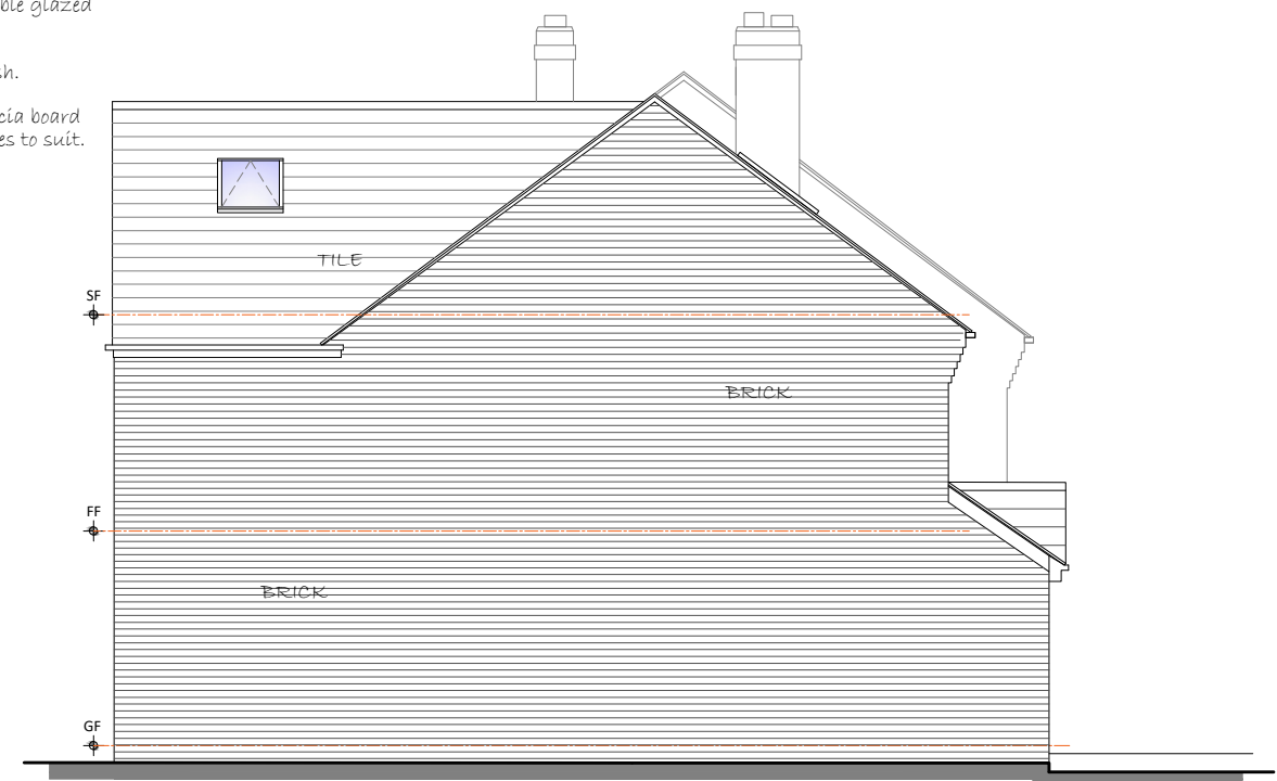
PROPOSED EAST (SIDE) ELEVATION SCALE - 1:100
