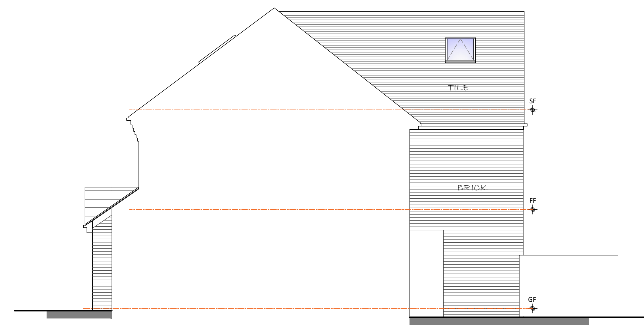
PROPOSED WEST (SIDE) ELEVATION SCALE - 1:100
