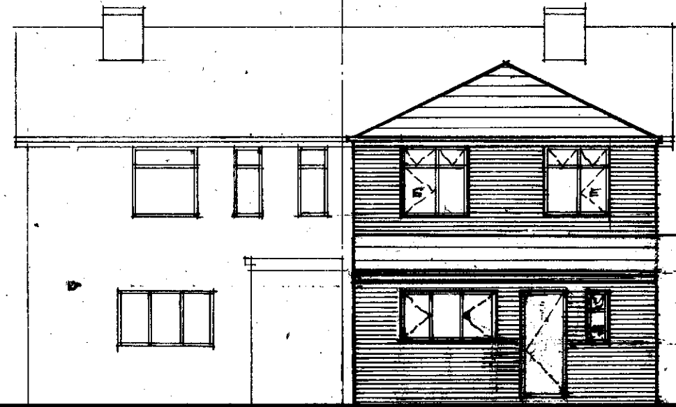
REAR 1:100
