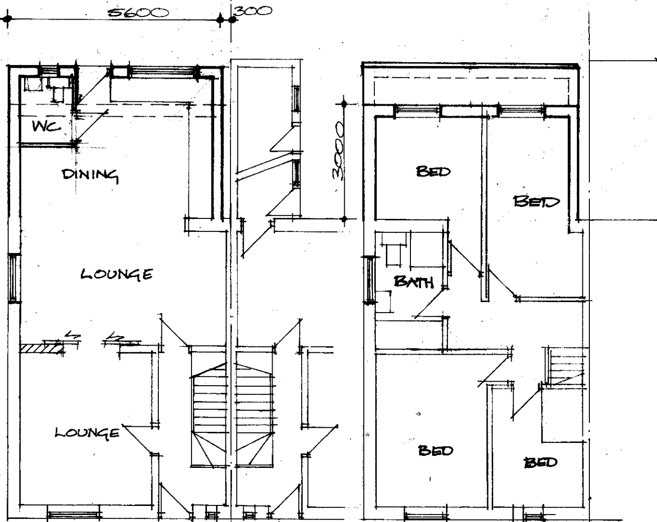
FIRST 1:100
