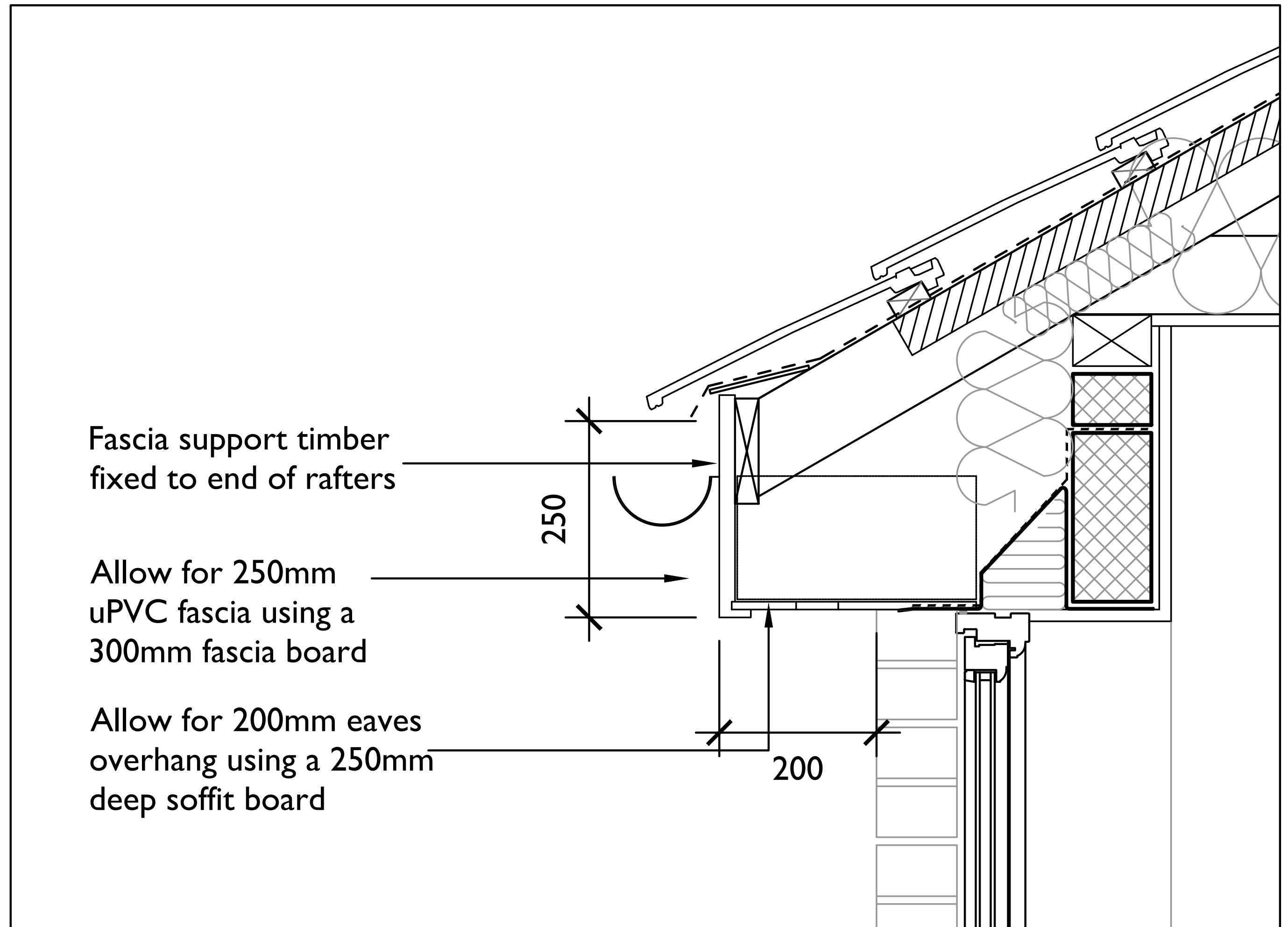
Eaves Detail 1/20
