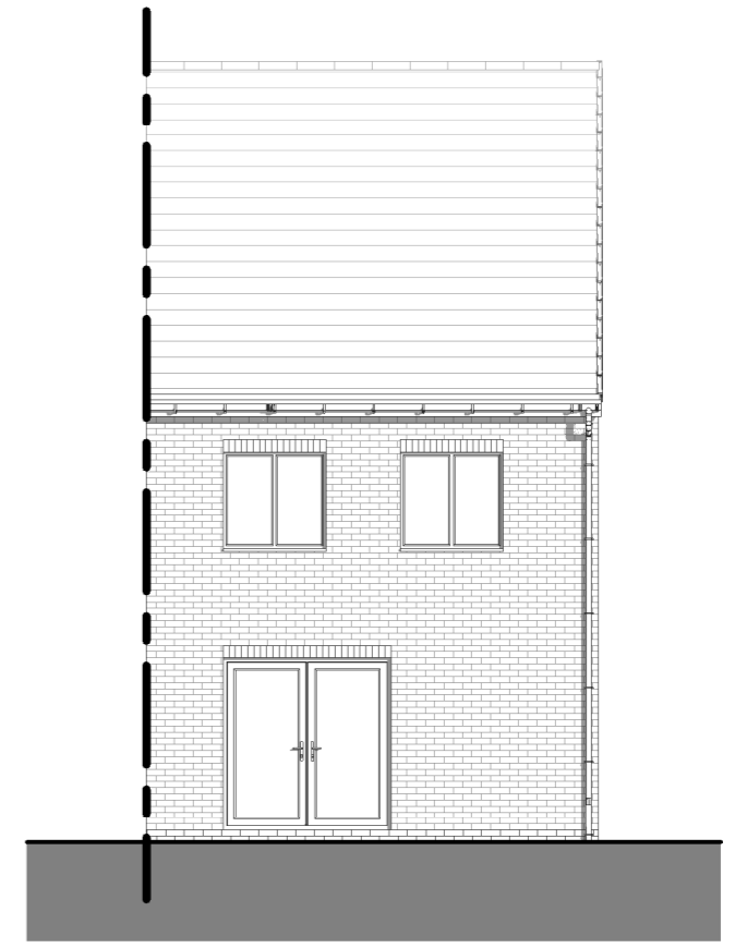
REAR
