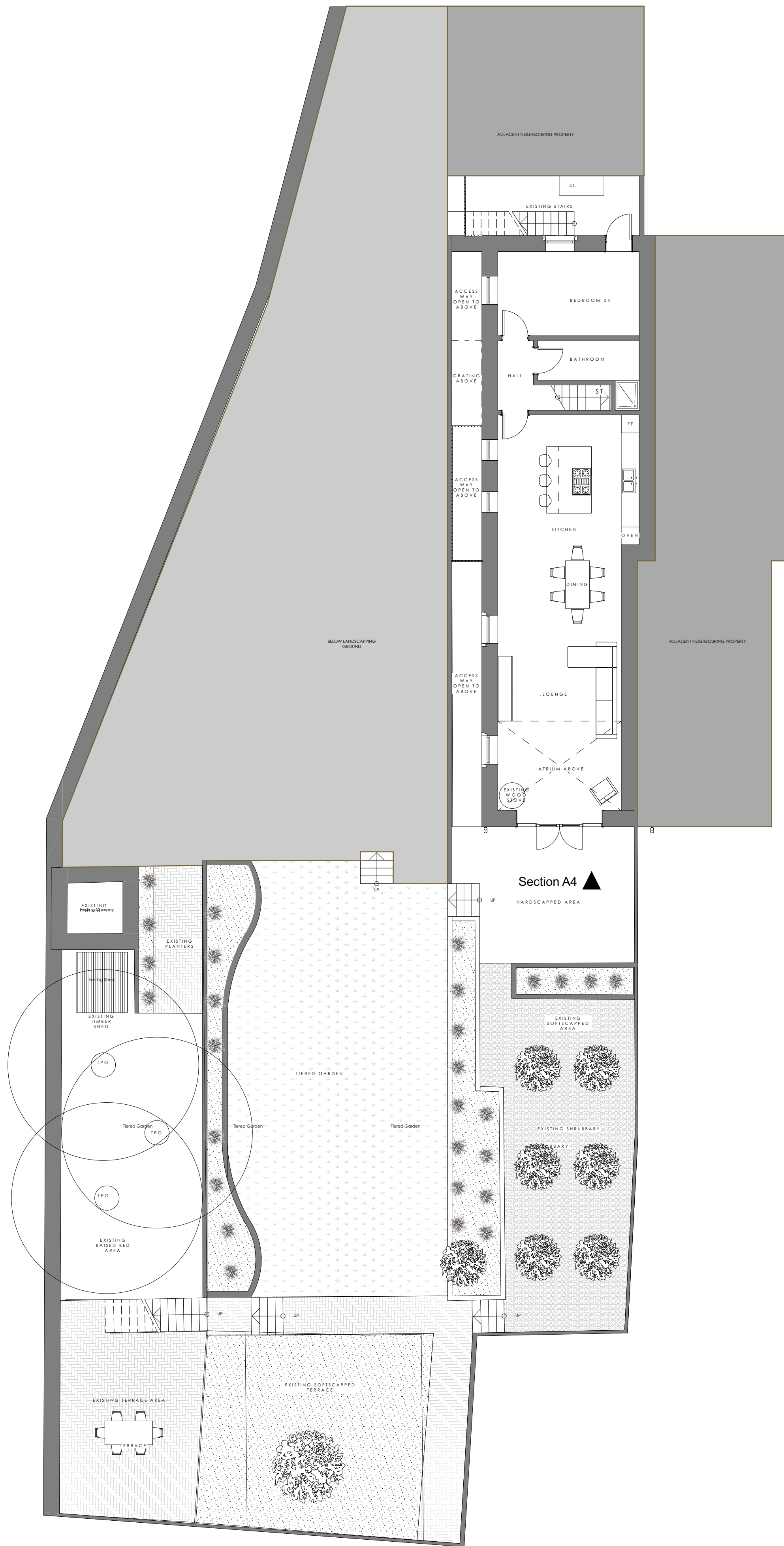
EXISTING LOWER GROUND FLOOR
