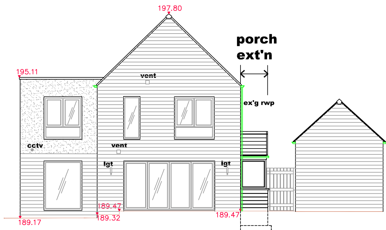
REAR ELEVATION (1:100) north west facing)
