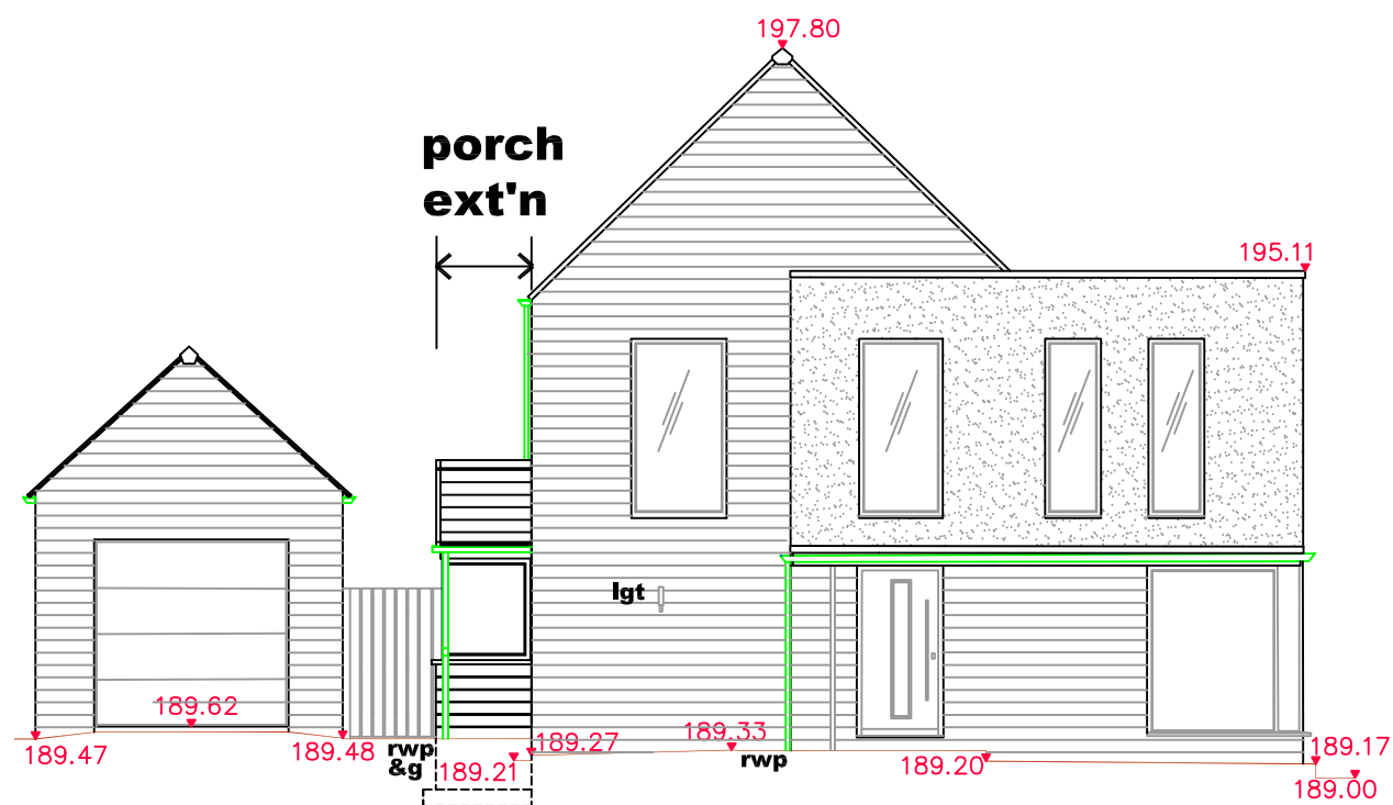
FRONT ELEVATION (1:100) (south east facing)
