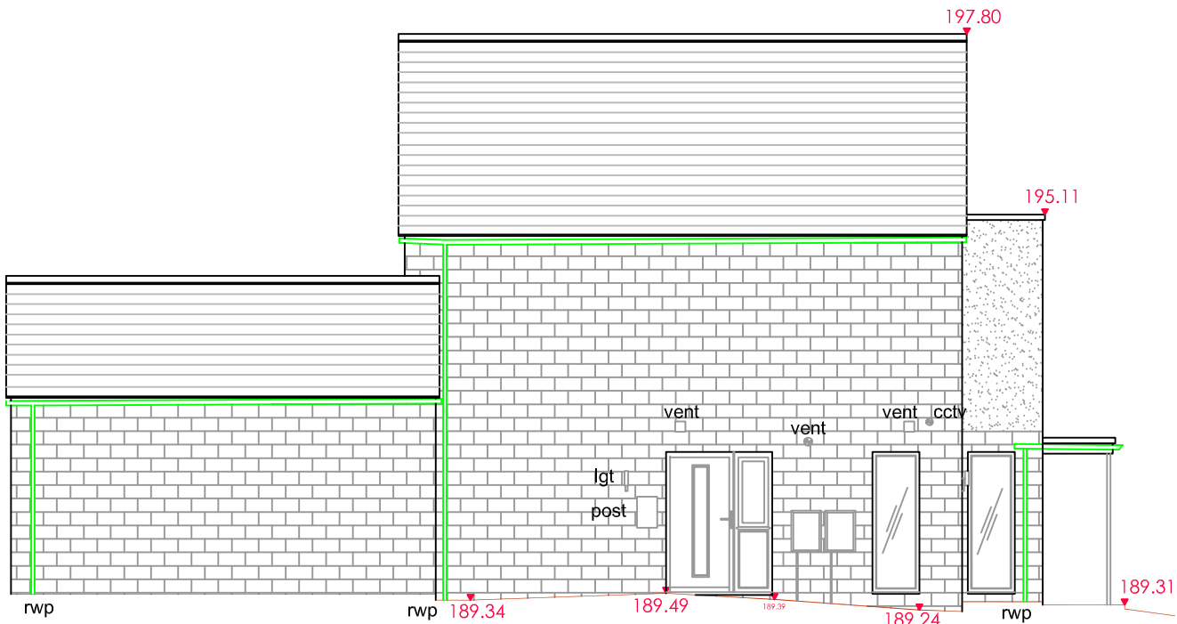
SIDE ELEVATION (1:100) (south west facing)
