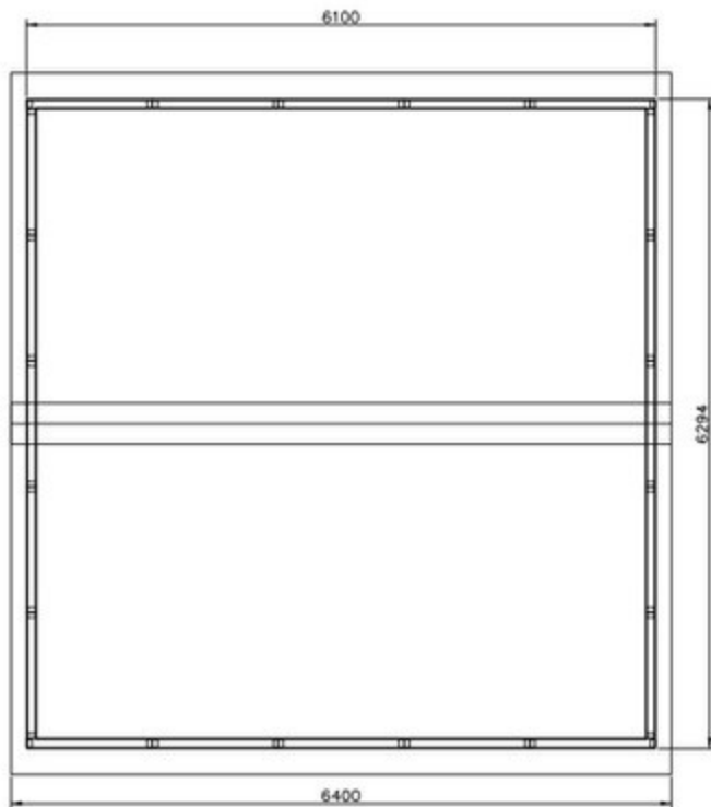
PLAN VIEW
