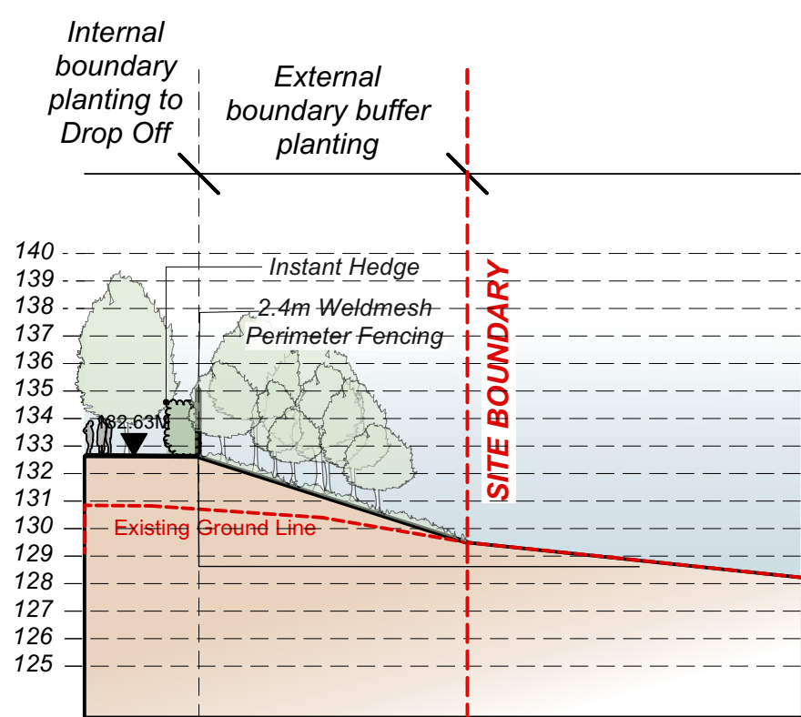
Site section D-D*: Buffer Planting Year 5 Scale 1:250
