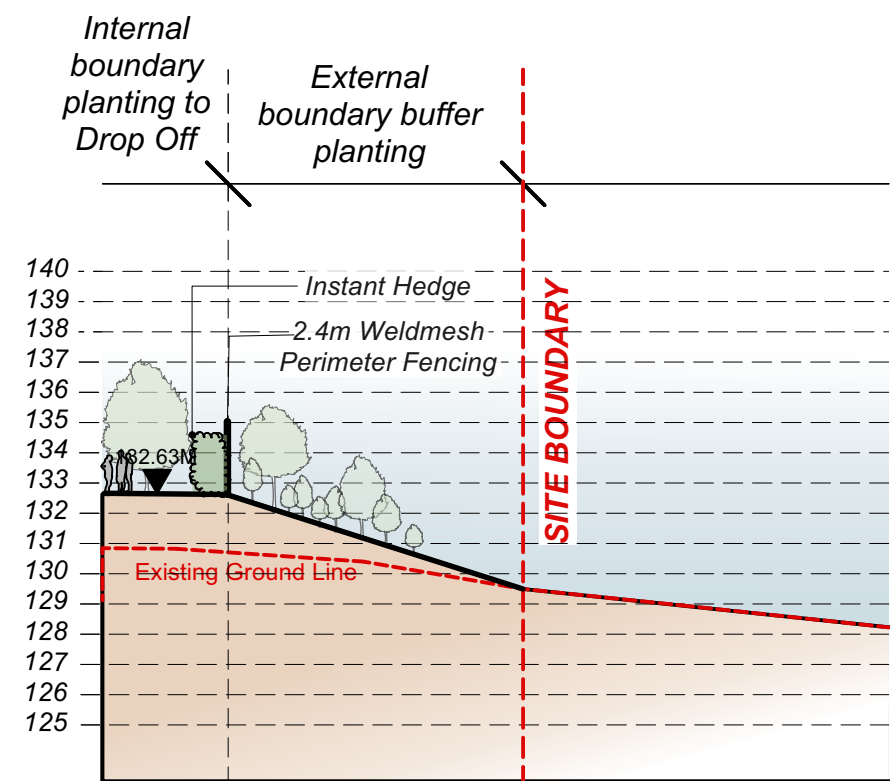
Site section D-D*: Buffer Planting Year 1 Scale 1:250
