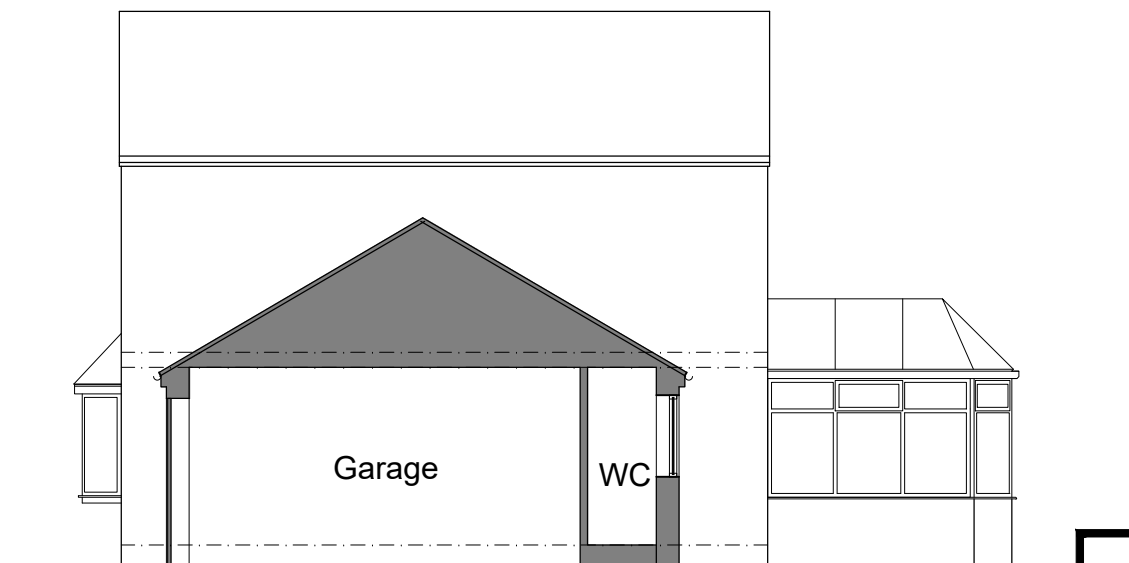
Side Elevation/Garage Section - Existing
