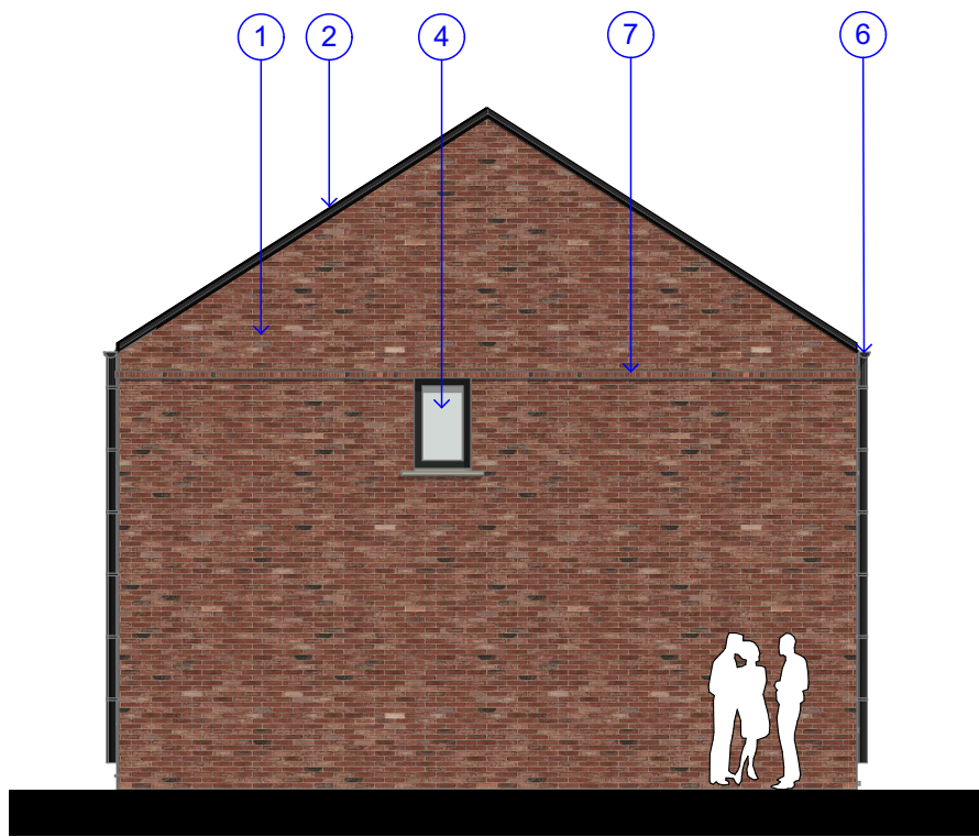
E-03 Elevation
