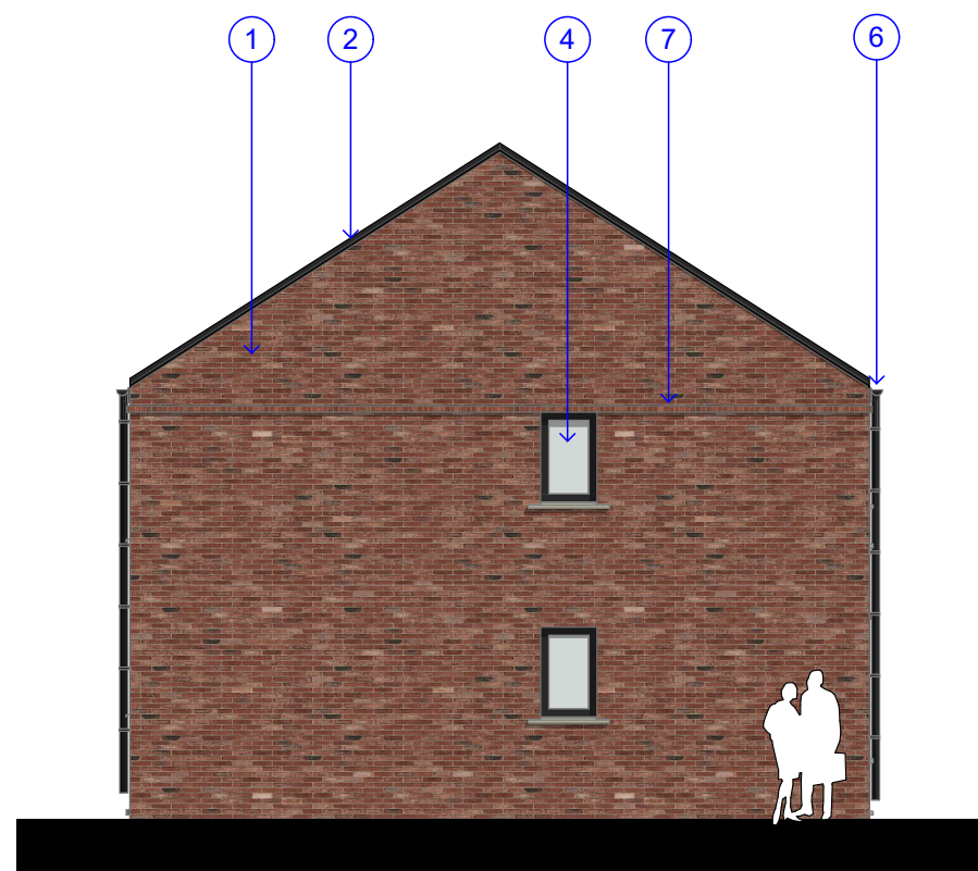
E-03 Elevation
