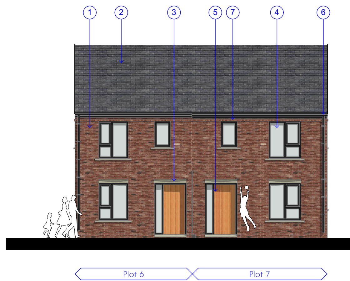
E-01 Elevation
