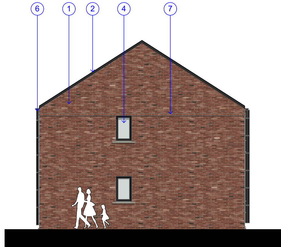
E-04 Elevation
