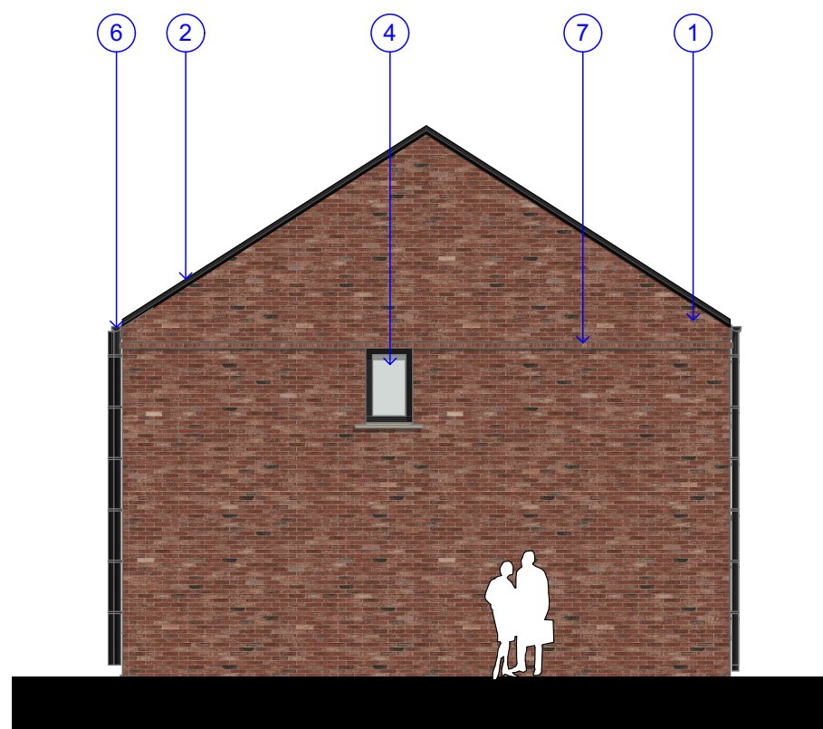
E-03 Elevation
