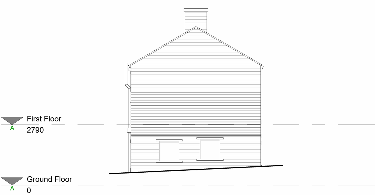
North East Elevation - Existing 1 : 100
