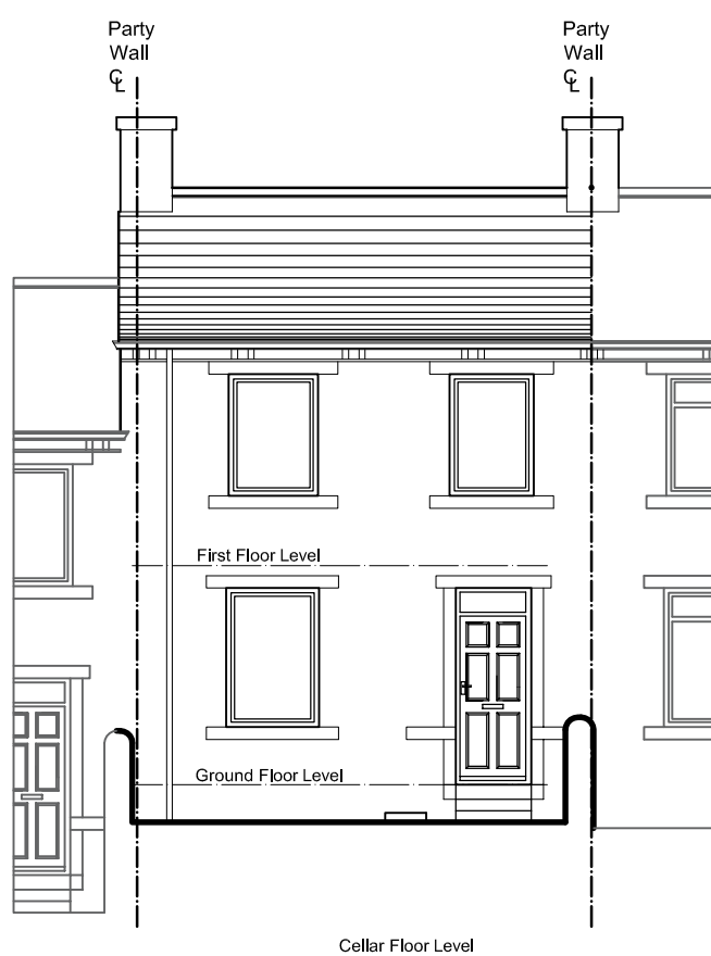
South East Elevation (front)
