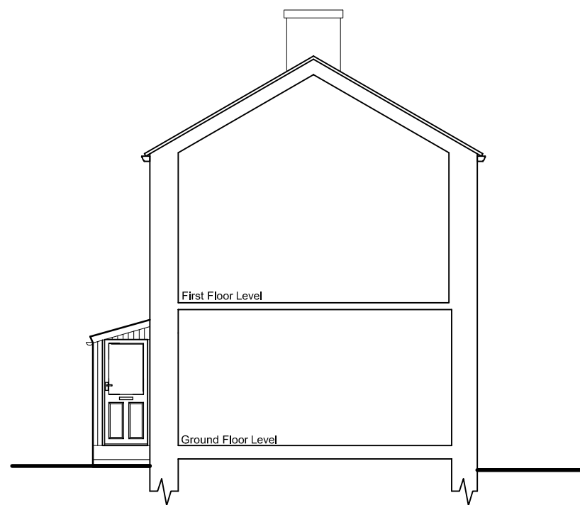
South West Sectional Elevation (side)
