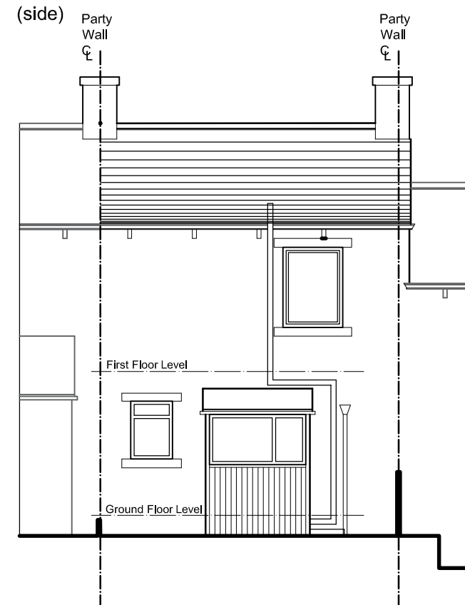
North West Elevation (rear)
