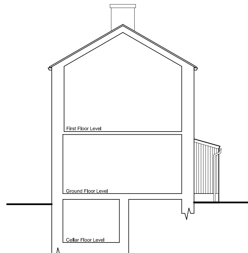
North East Sectional Elevation (side)
