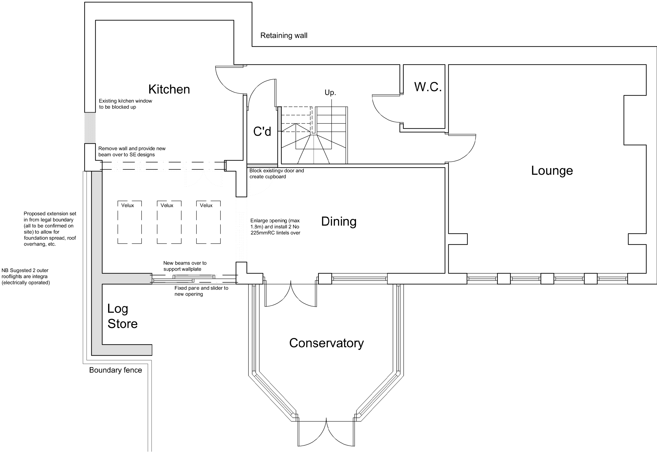
Lower Ground Floor Plan
