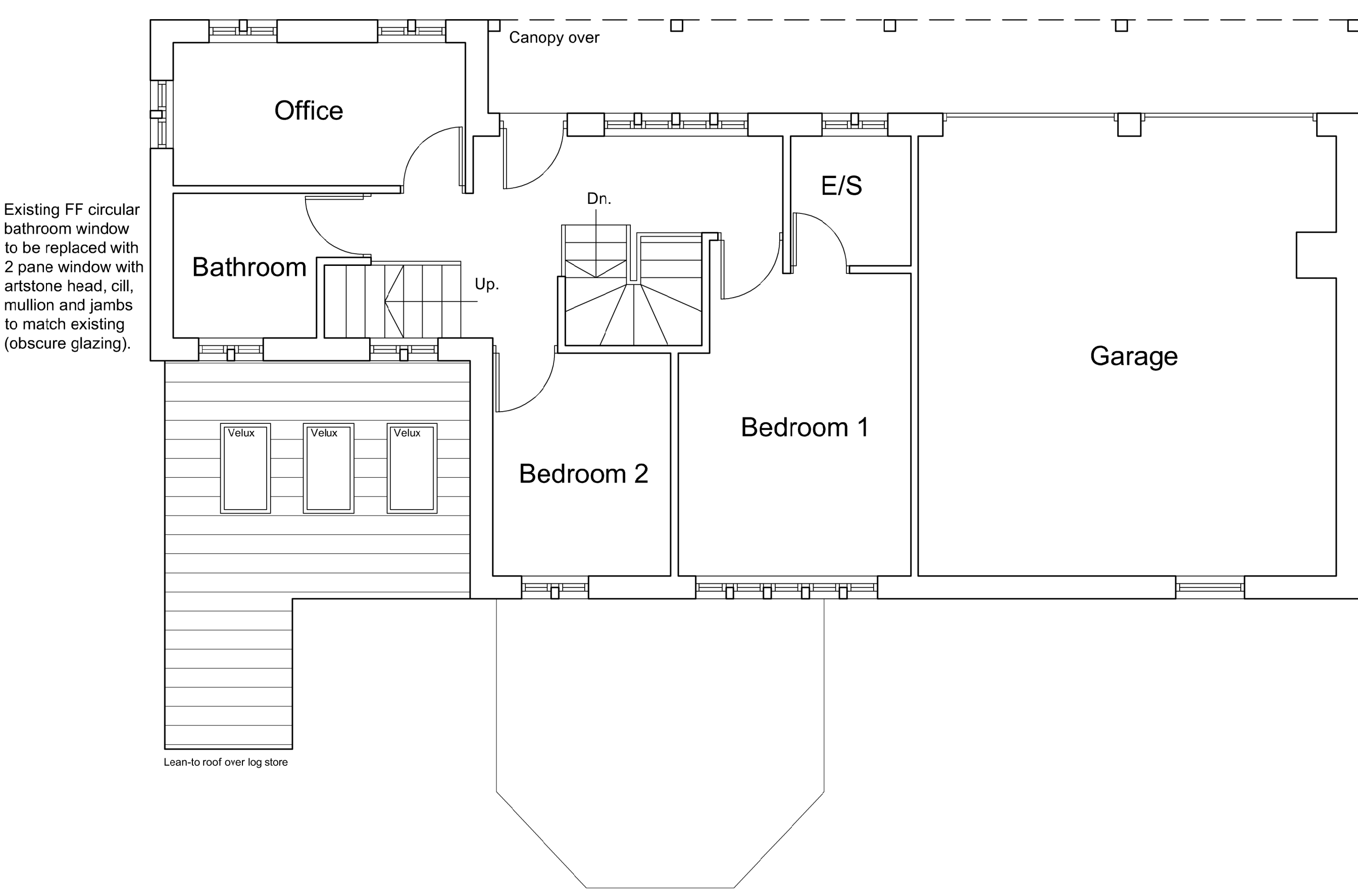
Upper Ground Floor Plan
