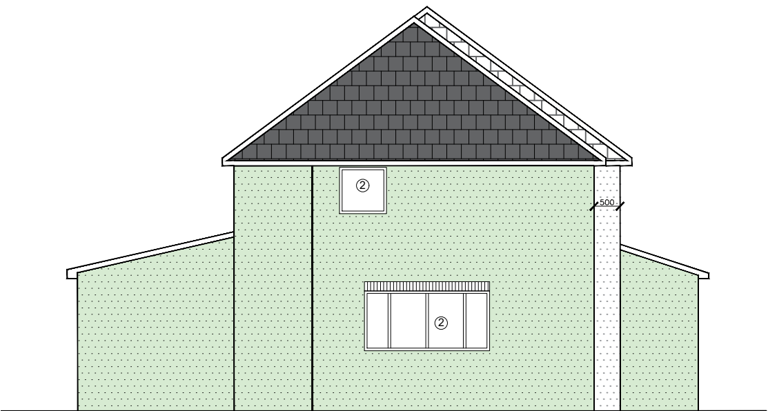
PROPOSED SIDE ELEVATION (South West)
