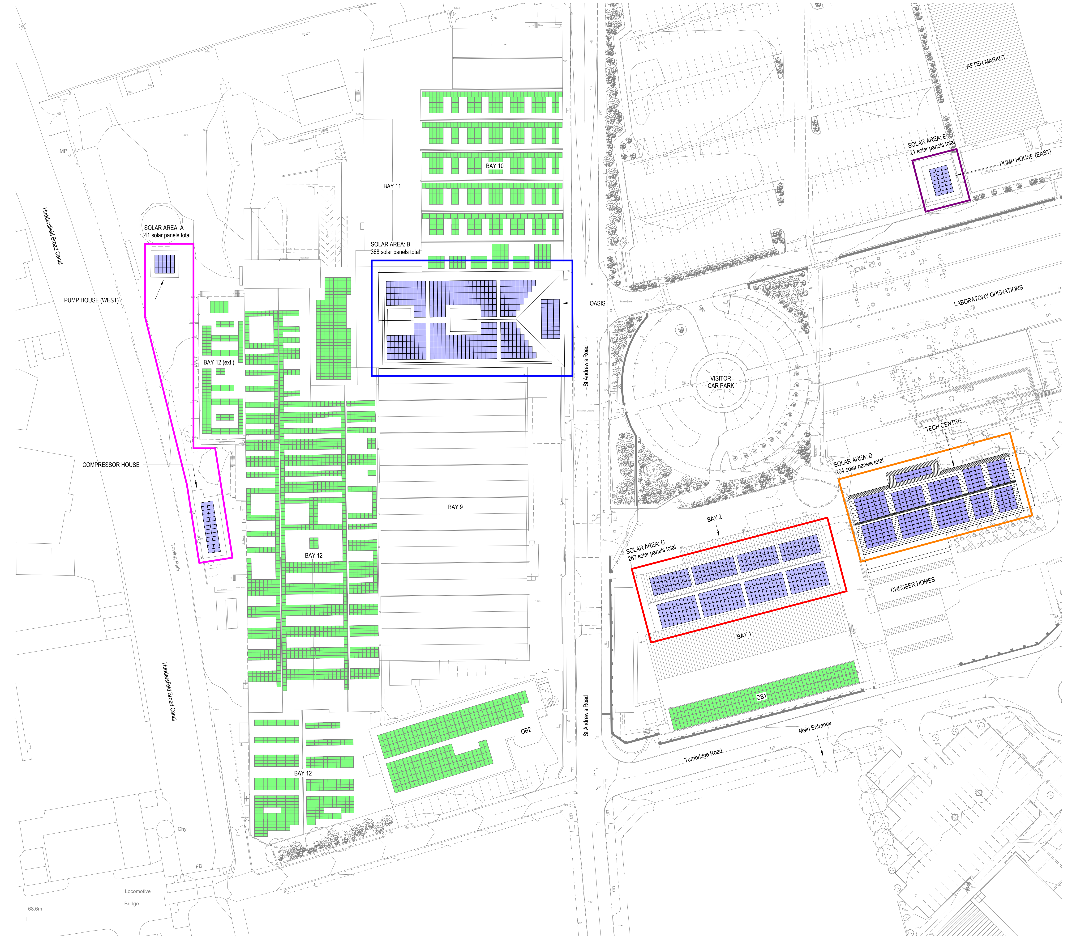
SITE PLAN - AS PROPOSED 1 : 500
