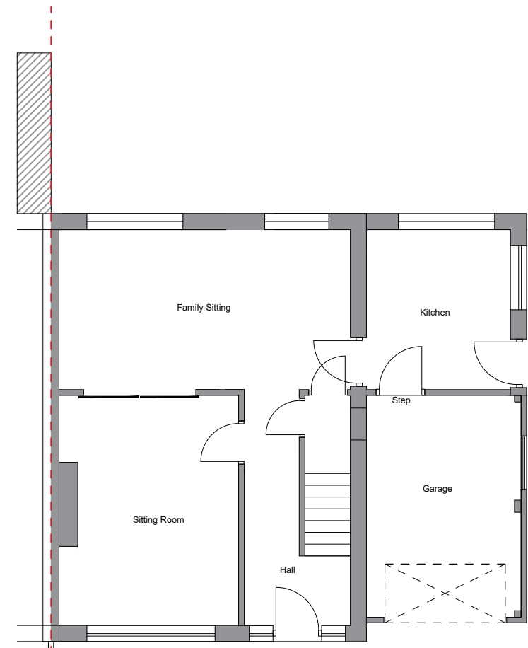
EXISTING GROUND FLOOR PLANS
