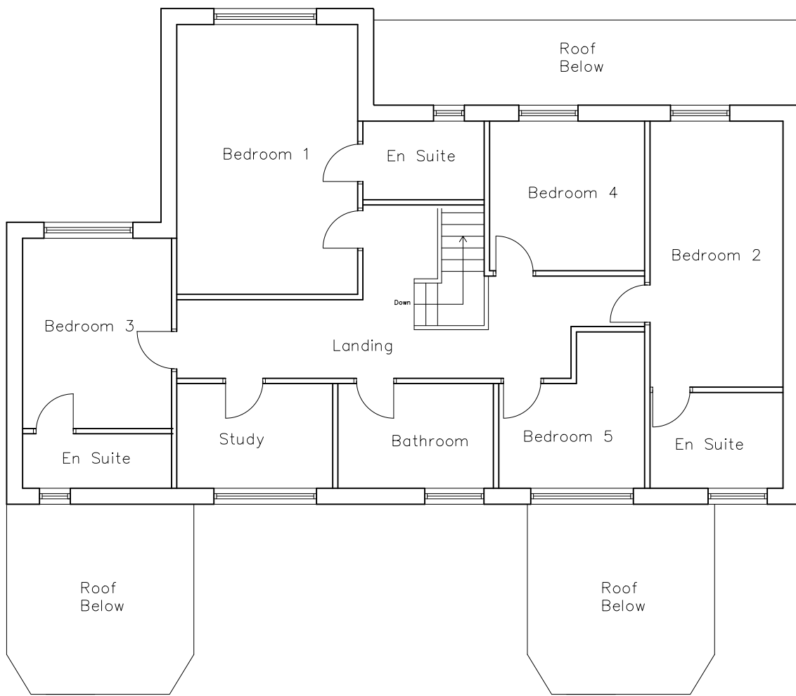
First Floor as Existing
