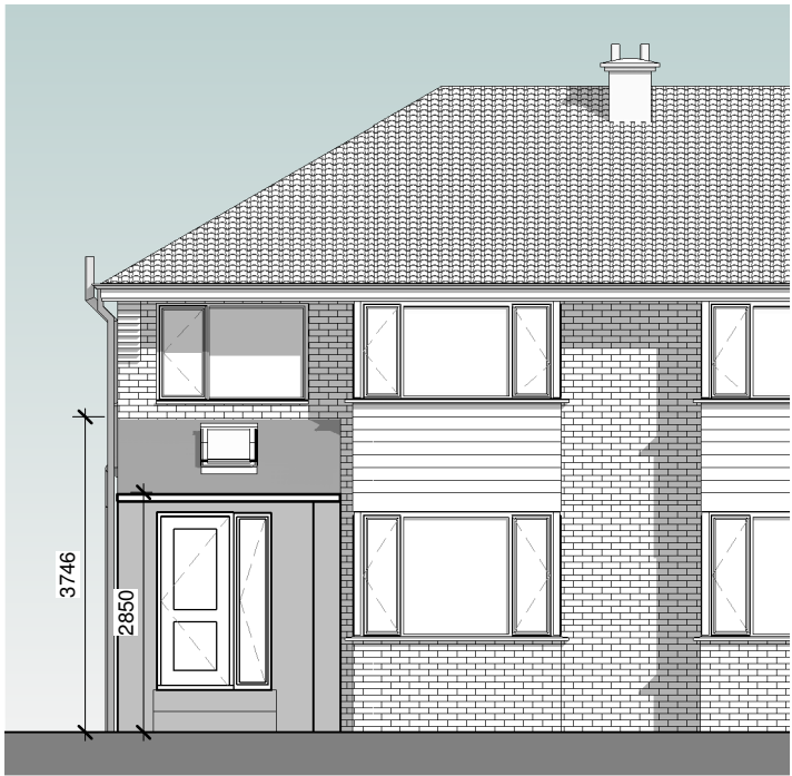
FRONT ELEVATION PORCH 1 : 100
