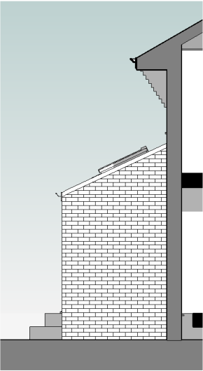
SIDE ELEVATION ADJACENT BAY WINDOW 1 : 100
