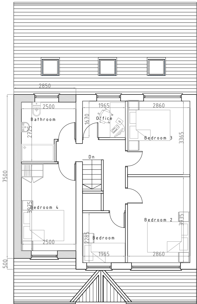
PROPOSED FF PLAN 1:100
