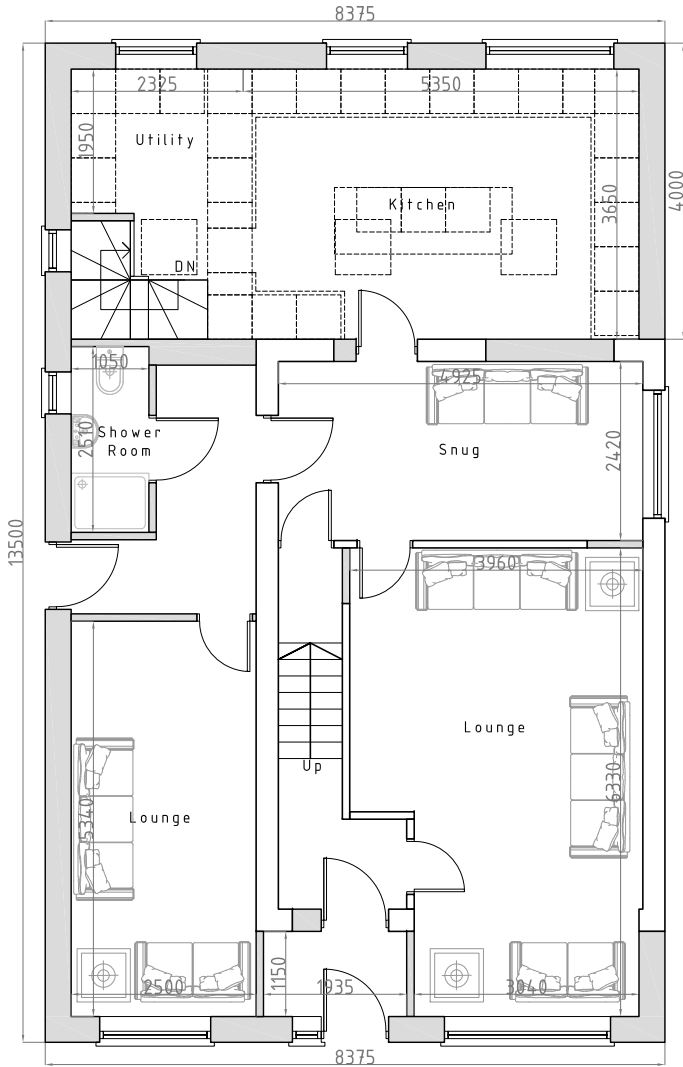
PROPOSED GF PLAN 1:100
