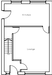
EXISTING GF PLAN 1:200
