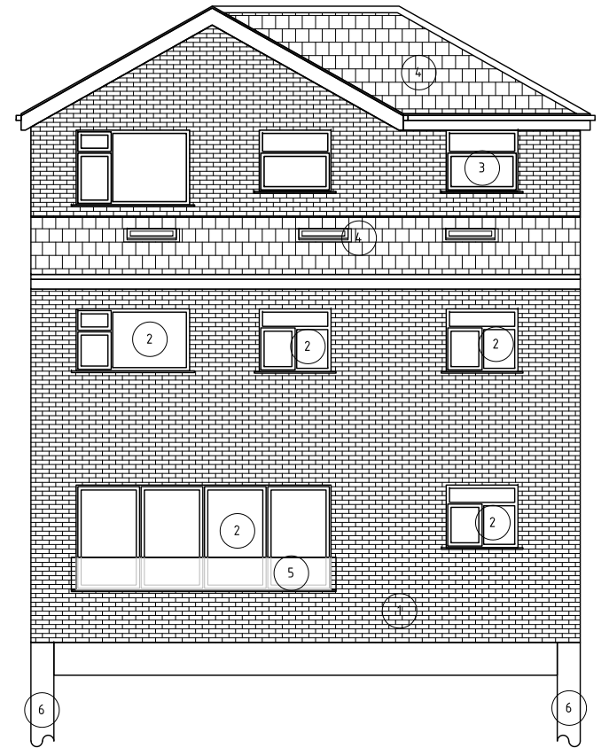
PROPOSED REAR ELEV 1:100
