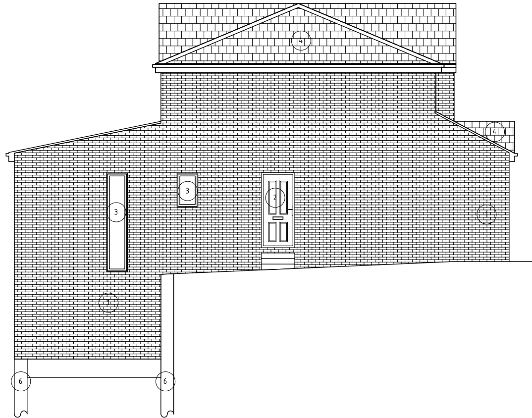
PROPOSED SIDE ELEV 1:100
