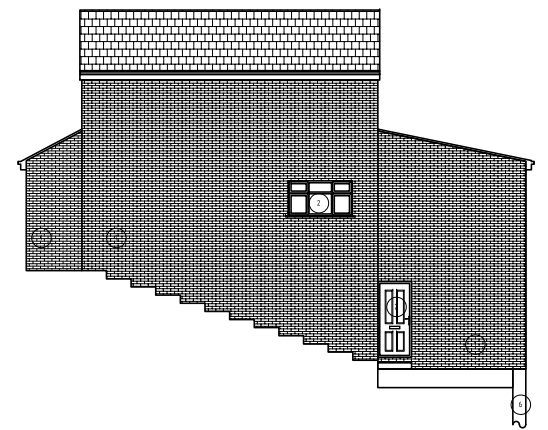
PROPOSED OTHER SIDE ELEV 1:200
