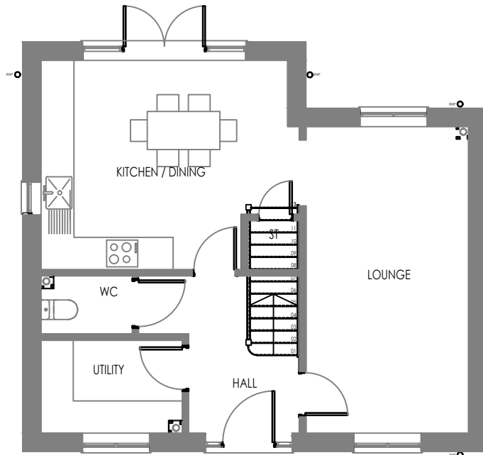
Ground floor 1:100
