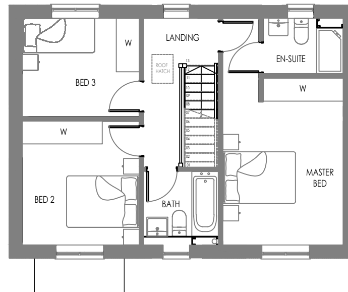
First floor 1:100
