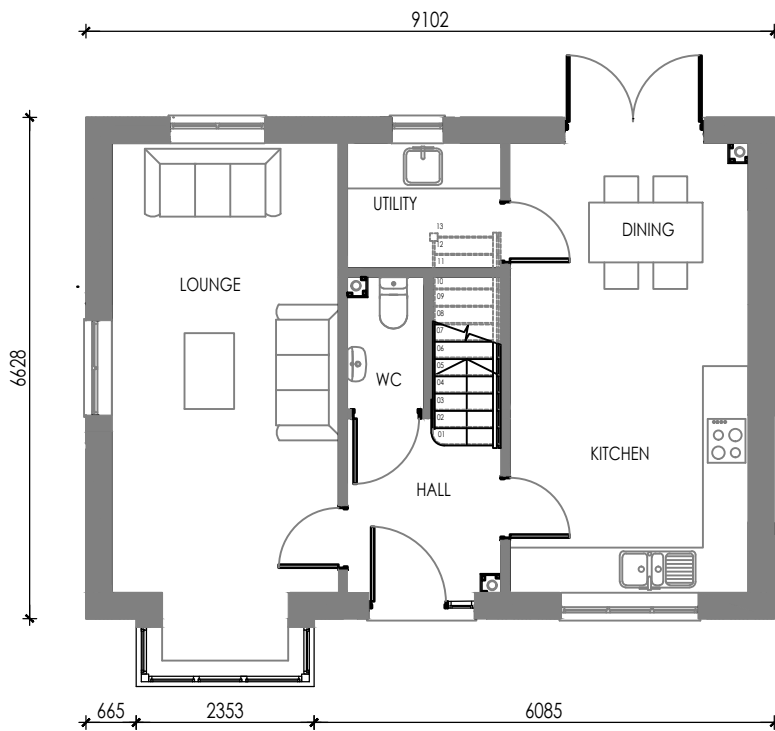
Ground floor 1:100
