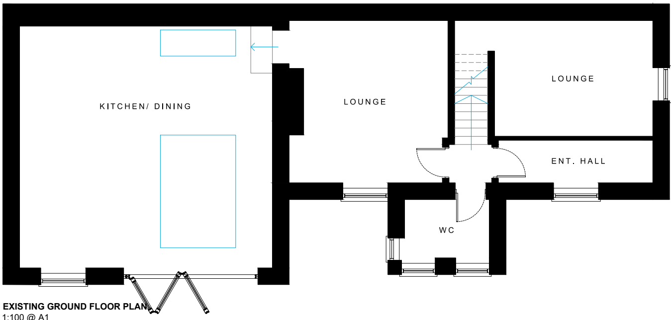
EXISTING GROUND FLOOR PLAN 1:100 @ A1
