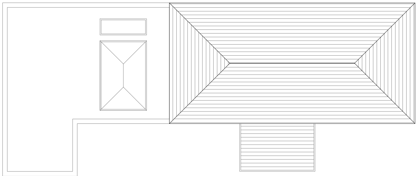
PROPOSED ROOF PLAN 1:100 @ A1
