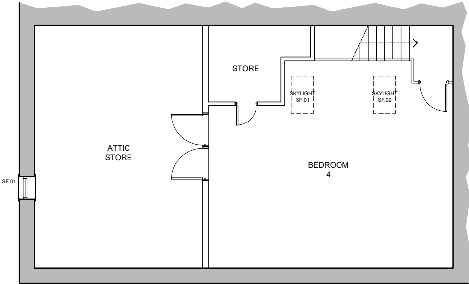
ATTIC FLOOR
