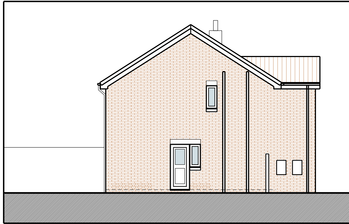
East Elevation
