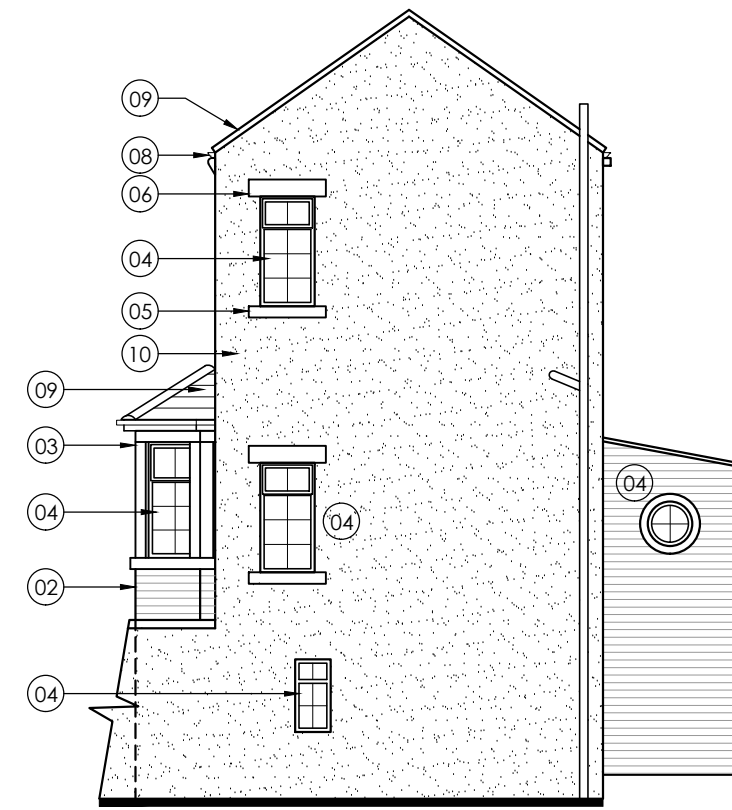
EAST ELEVATION
