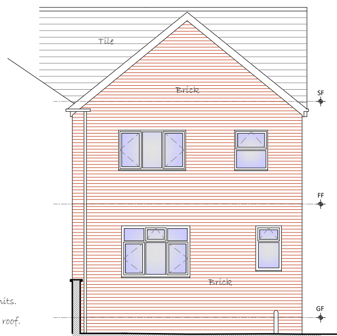
PROPOSED NORTH-EAST (REAR) ELEVATION SCALE - 1:100
