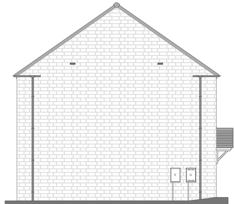
Left Elevation
