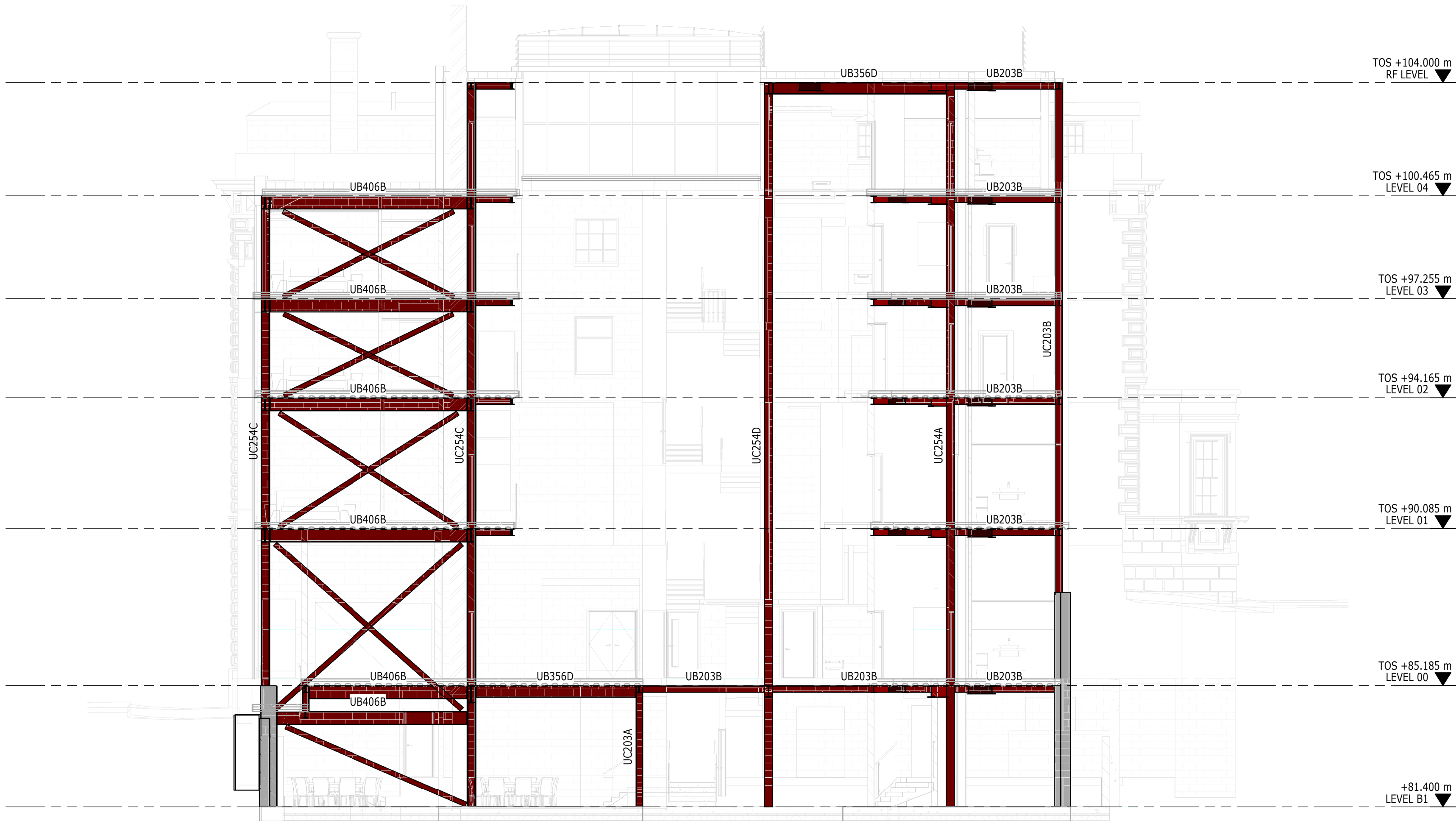
ELEVATION 1 : 100 BUILDING ELEVATION C
