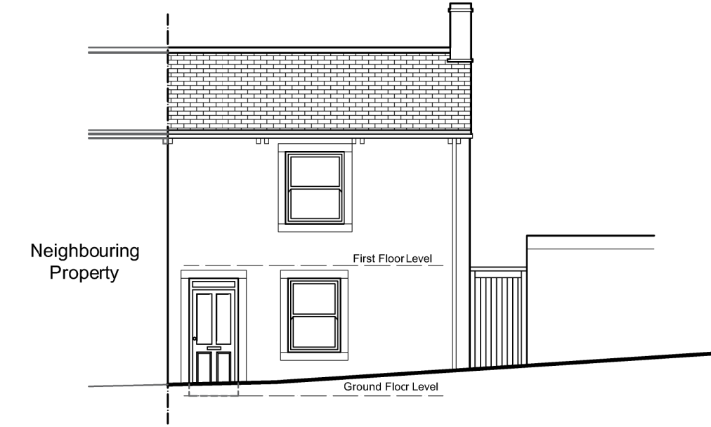
West Elevation
