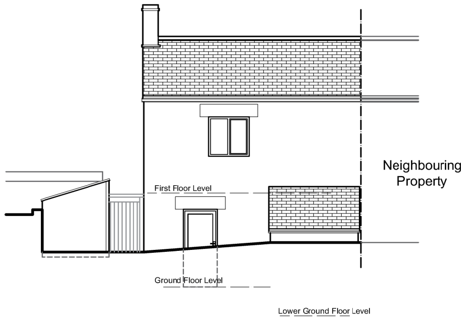
East Elevation
