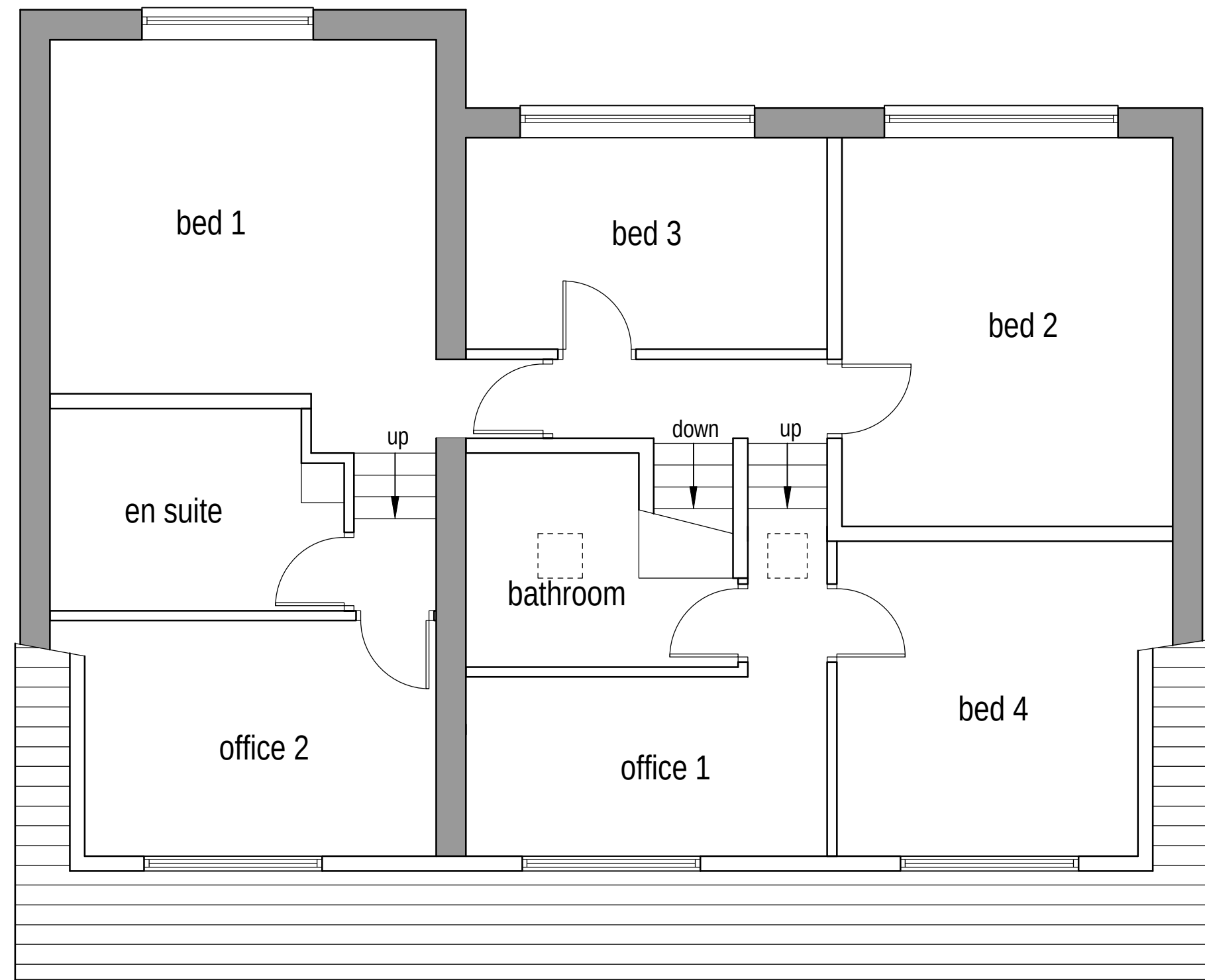
Proposed first floor layout (1:50)
