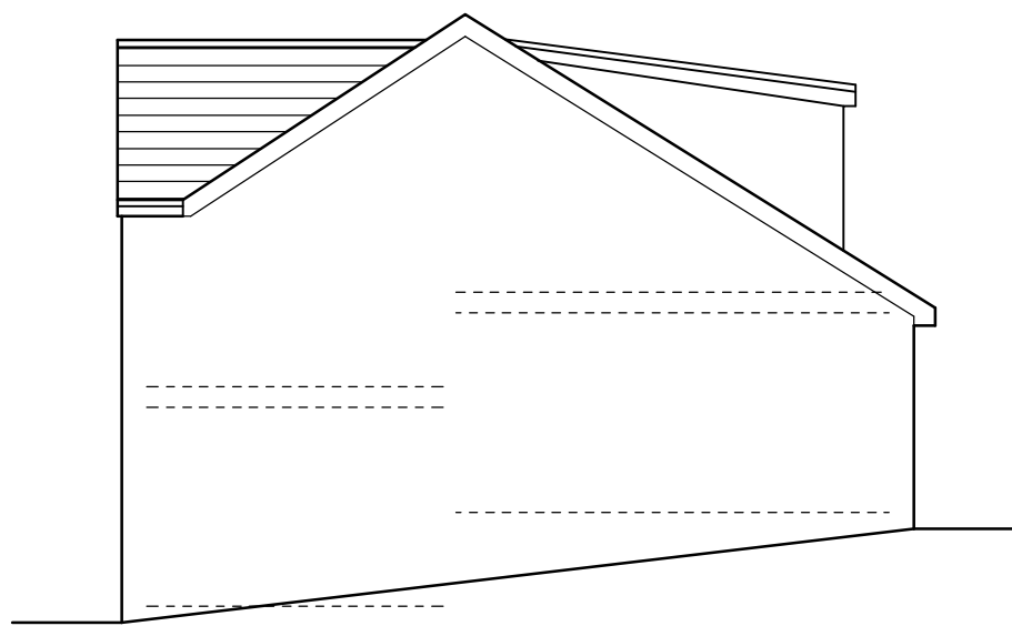
Proposed side/north facing elevation (1:100)
