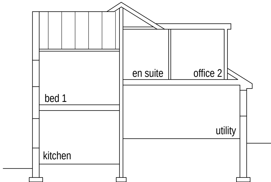
Proposed cross section (1:100)
