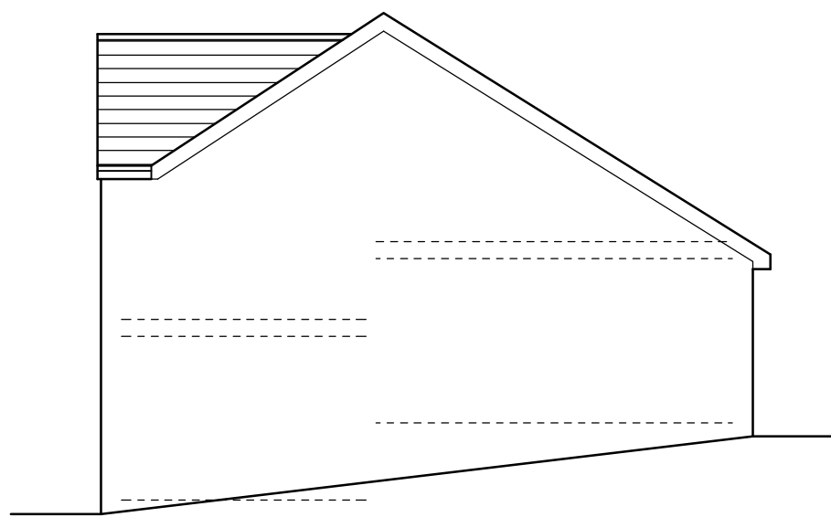
Existing side/north facing elevation (1:100)
