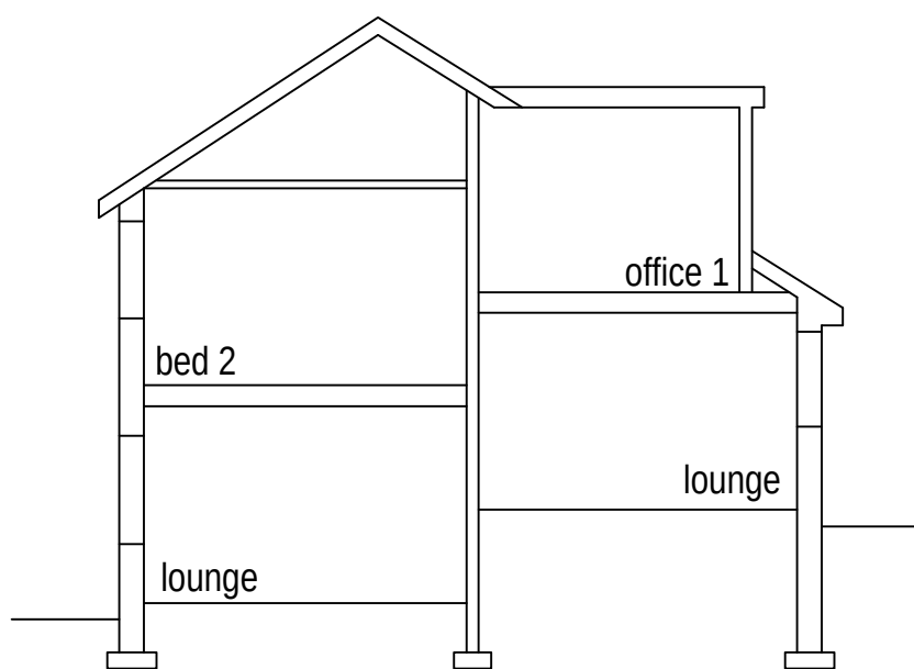
Proposed cross section (1:100)
