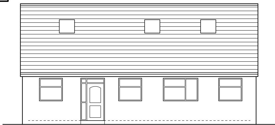
Existing front/west facing elevation (1:100)
