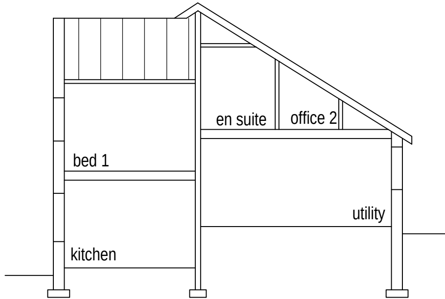
Existing cross section (1:100)
