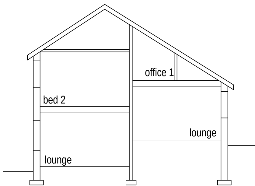
Existing cross section (1:100)
