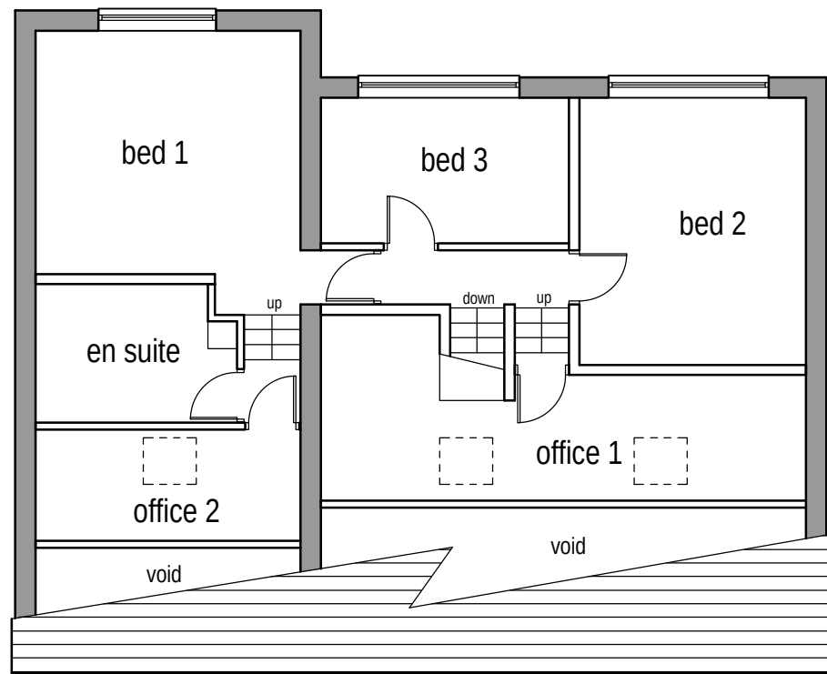
Existing first floor layout (1:100)
