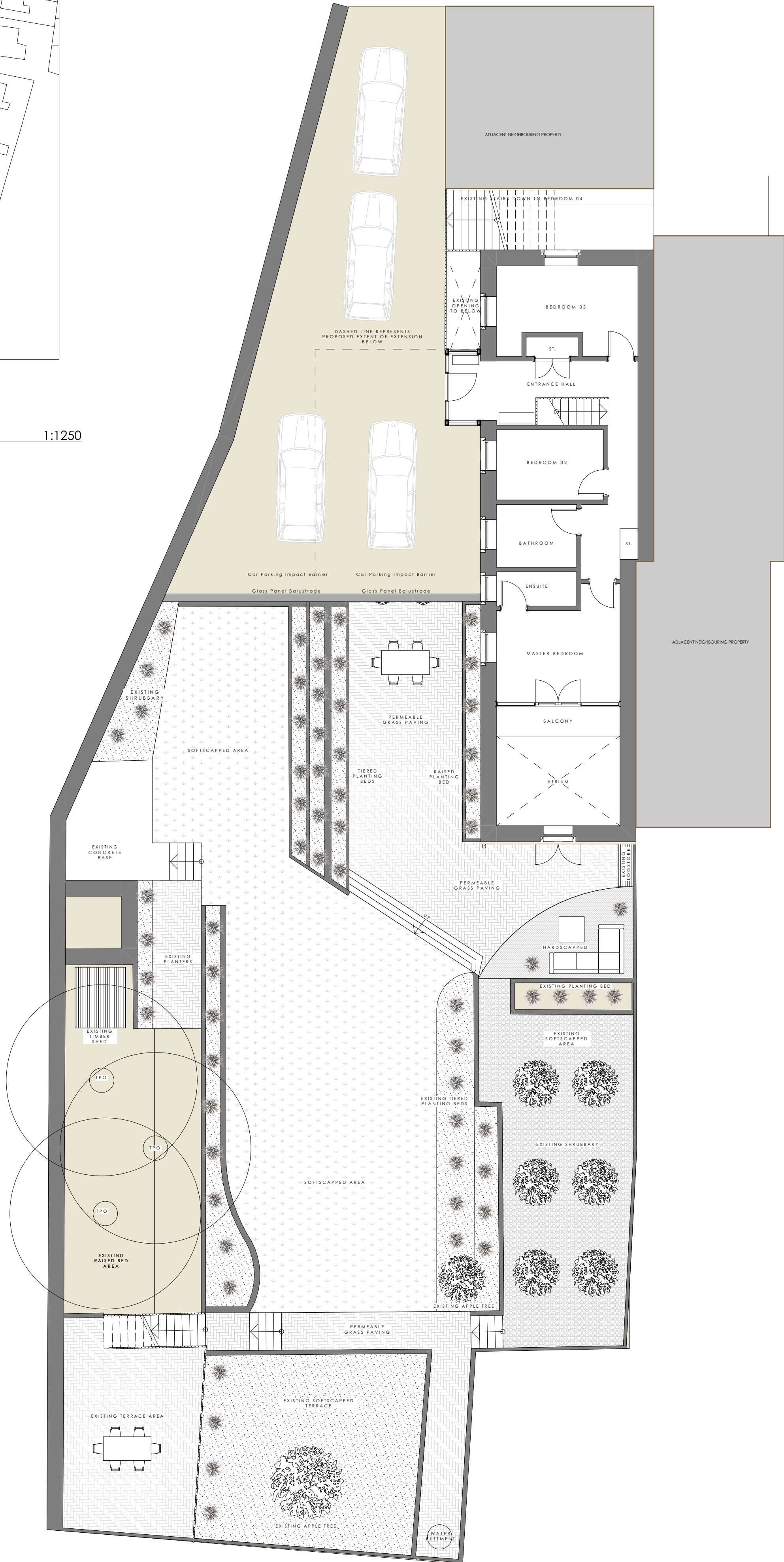
PROPOSED UPPER GROUND FLOOR
