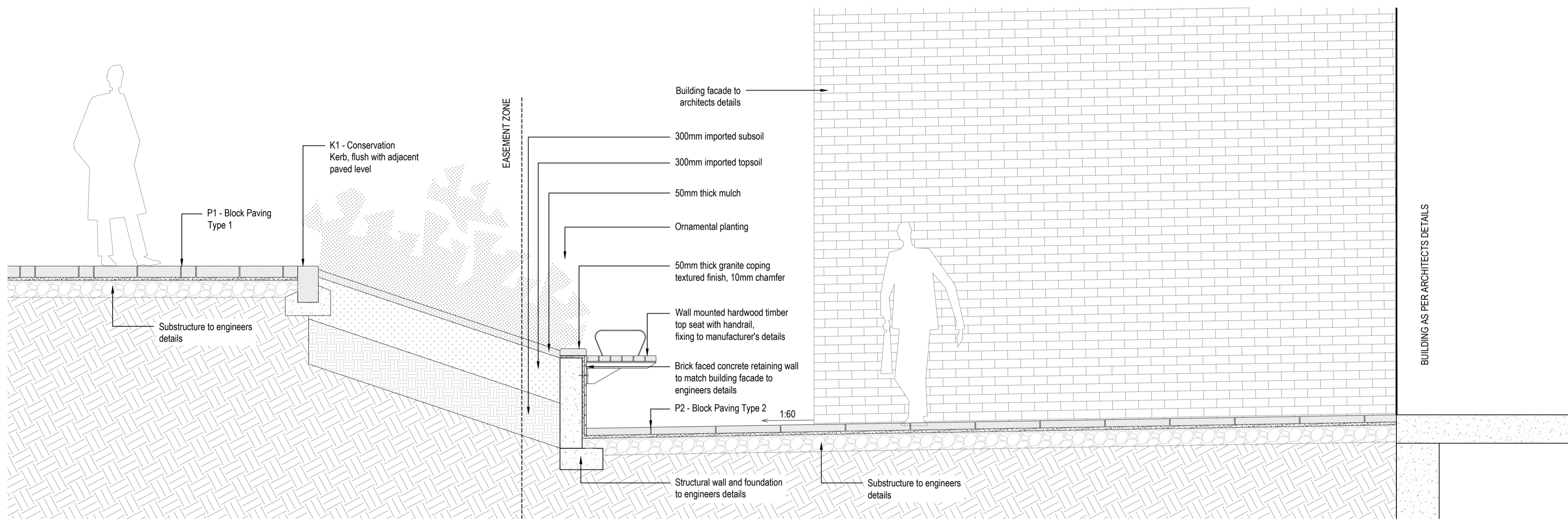
02 20011 SECTION 02 Scale 1: 20 @A1
