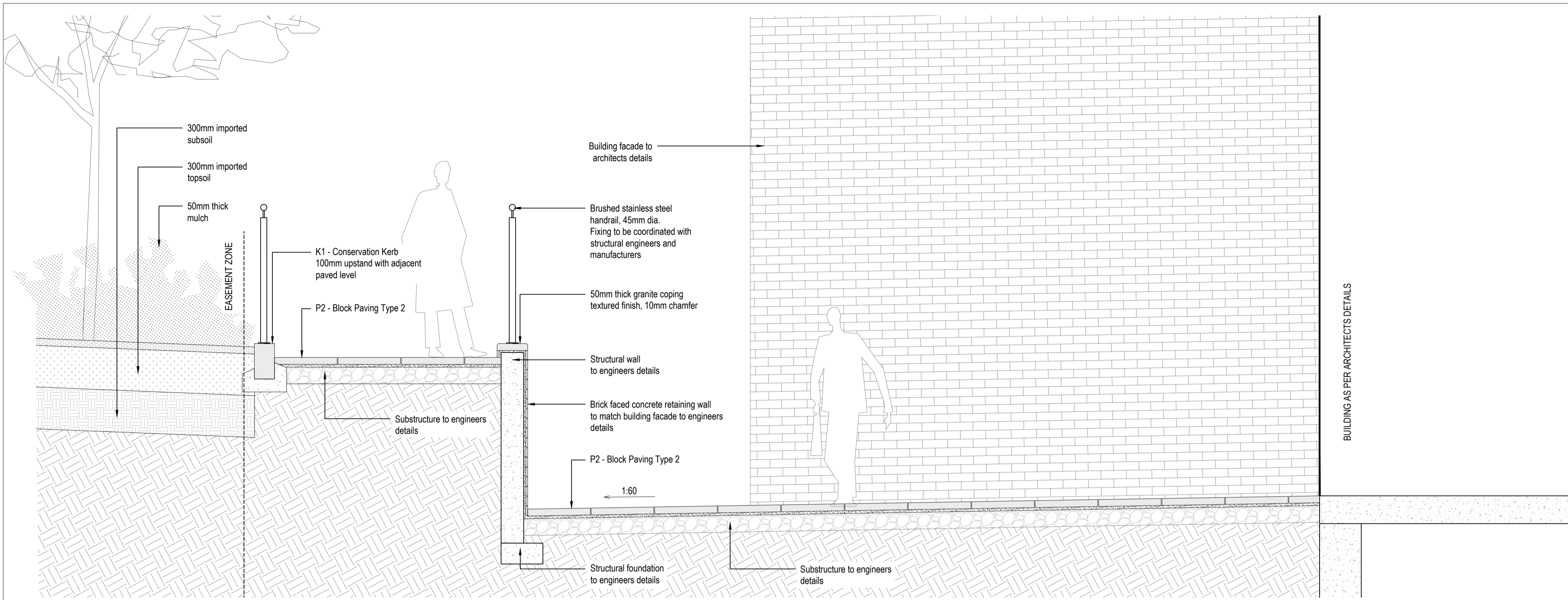
01 20011 SECTION 01 Scale 1: 20 @A1
