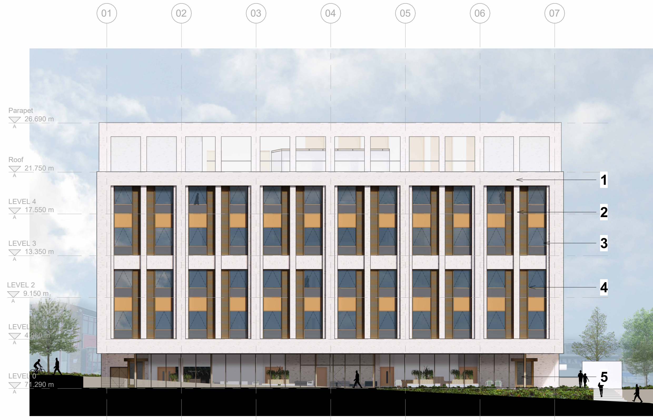
1 South Elevation
