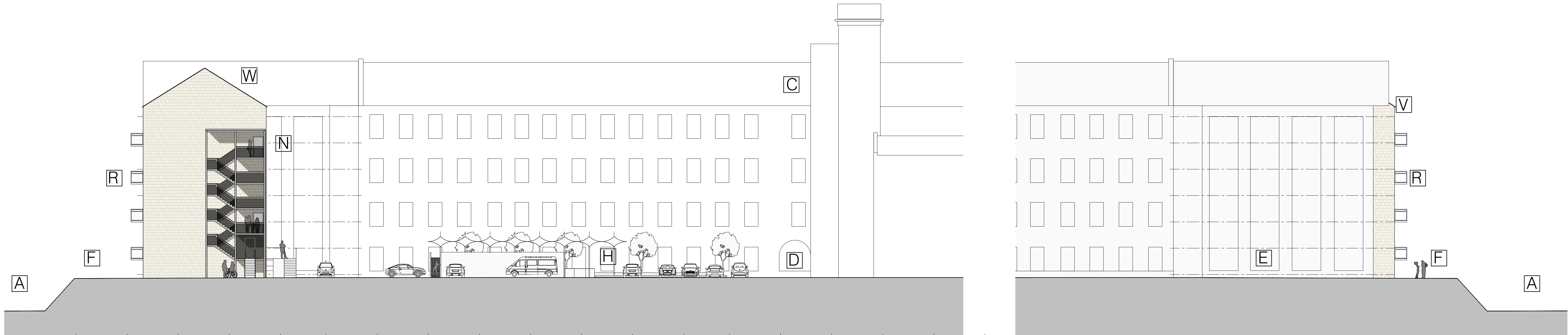
Side Elevation 1: 200
