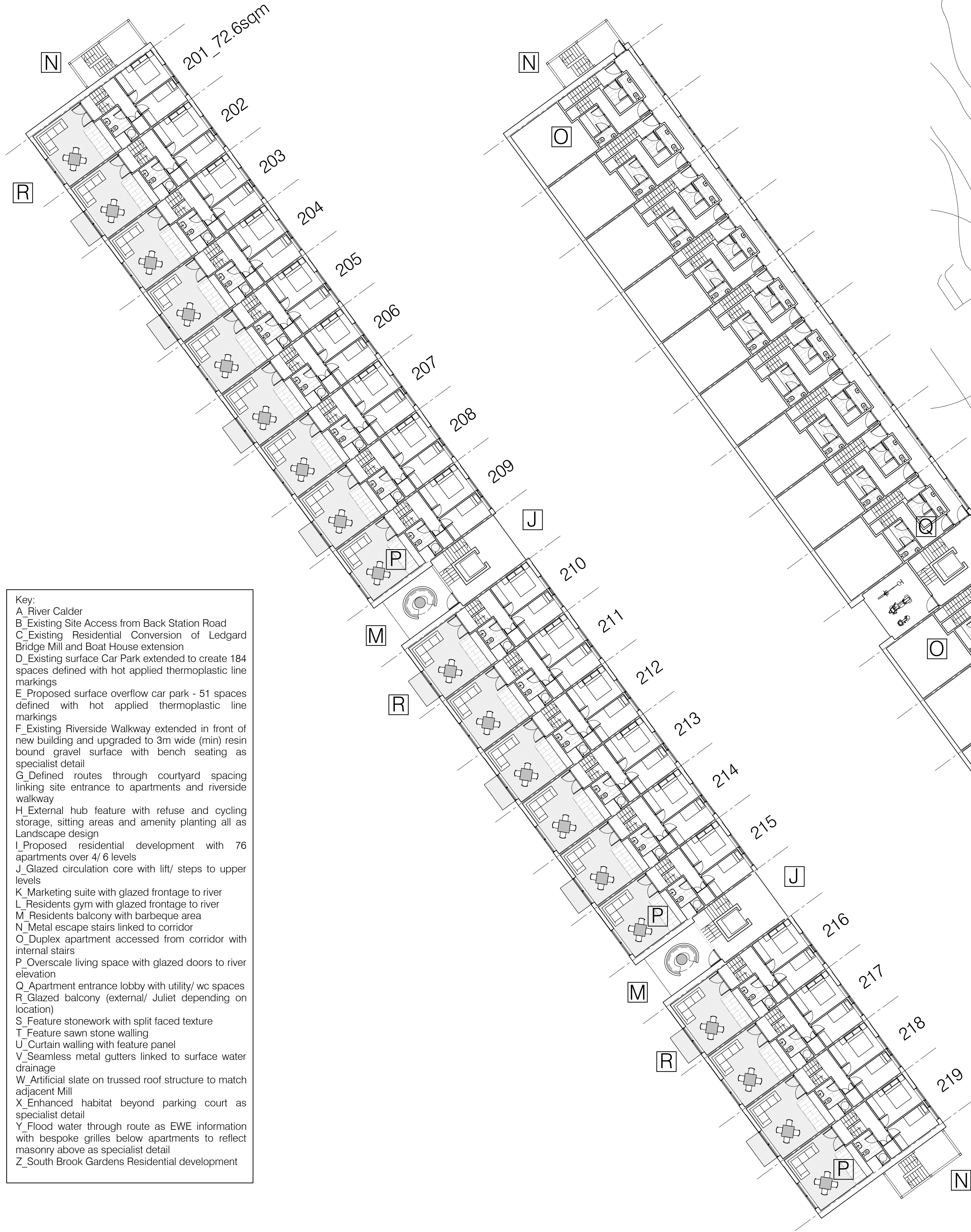
Second Floor Plan 1: 200
